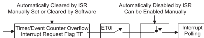
Interrupt Structure
