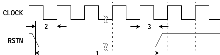
Figure 30: Power On Reset Timing
