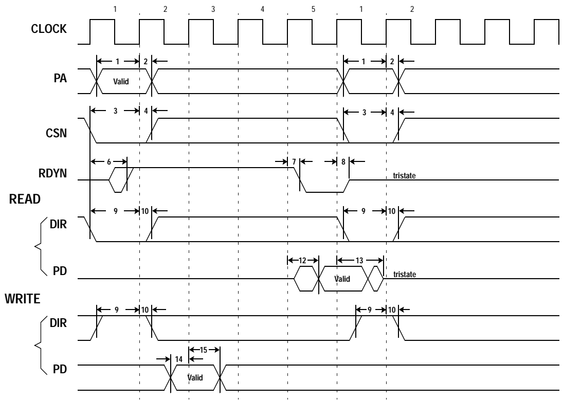
Figure 26: Microprocessor Interface Timing (PROCMODE[1]=0)
