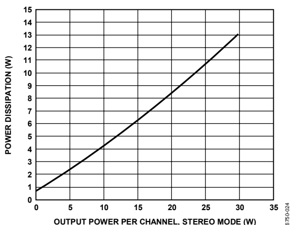
Figure 25. Power Dissipation vs. Output Power, 4 Ω
