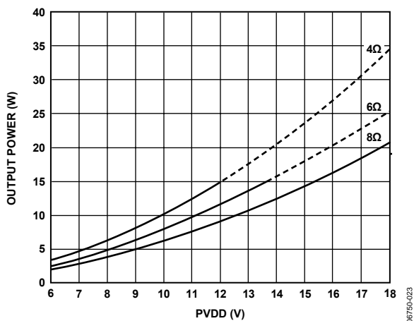
Figure 24. Output Power vs. PVDD, 20 dB THD + N
