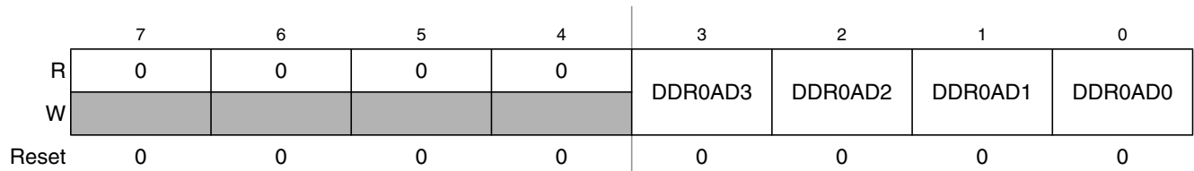
Figure 2-53. Port AD Data Direction Register (DDR0AD)
