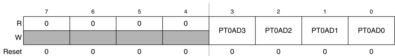
Figure 2-49. Port AD Data Register (PT0AD)
