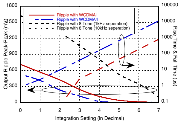
Output Ripple & Rise/Fall Time vs. Integration Setting Setting[Sci4,Sci3,Sci2,Sci1] in Decimal
