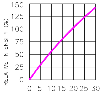
Fig.3 RELATIVE INTENSITY VS. FORWARD CURRENT
