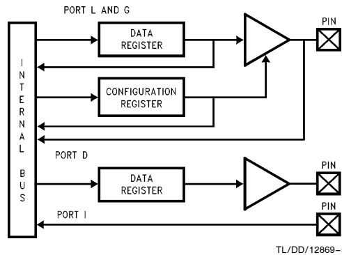
FIGURE 3. I/P Port Configurations
