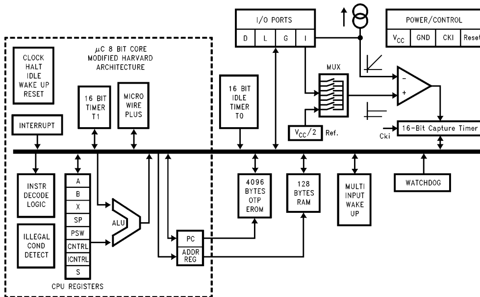
FIGURE 1. Block Diagram
