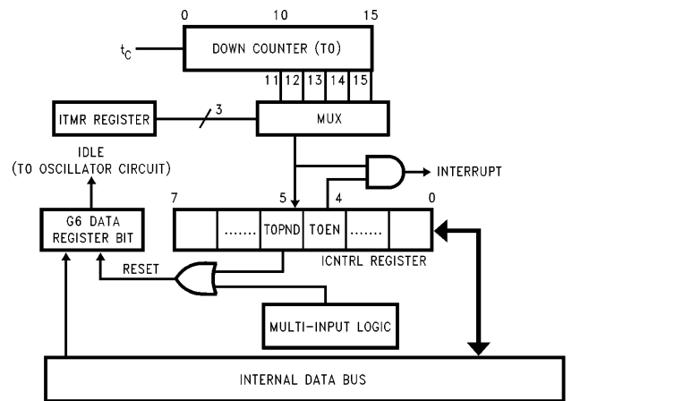
FIGURE 6. Functional Block Diagram for Idle Timer T0
