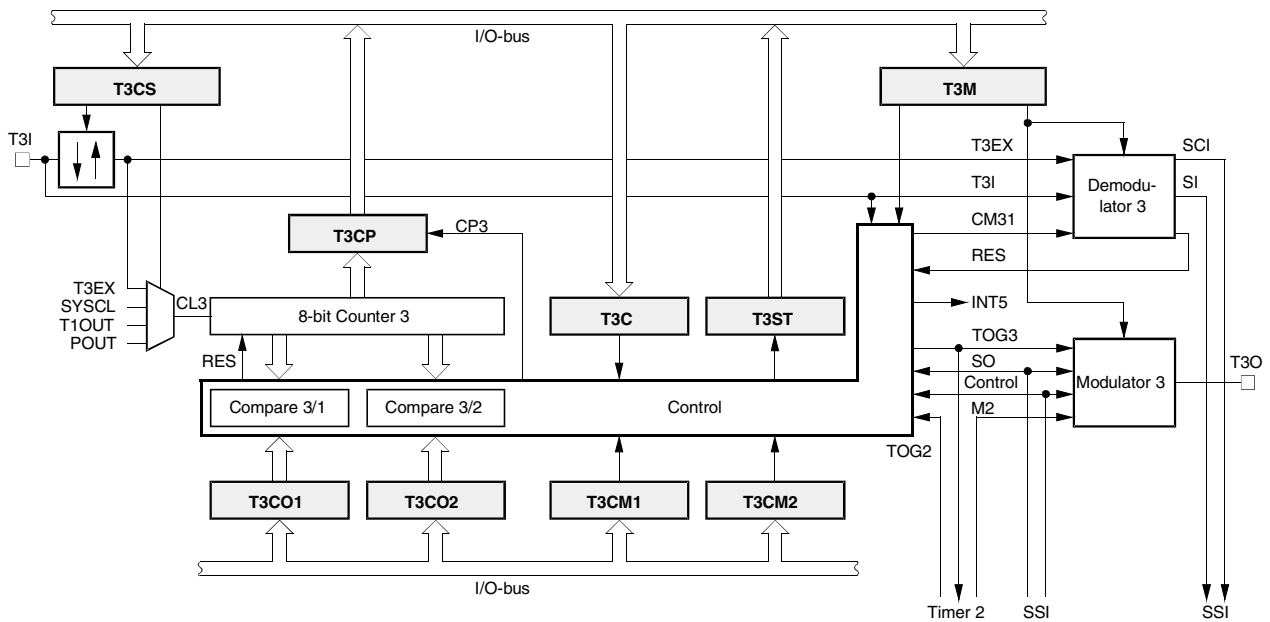
Figure 44. Timer 3
