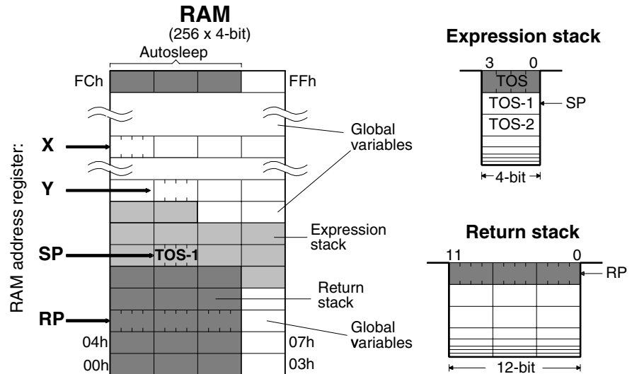
Figure 5. RAM Map
