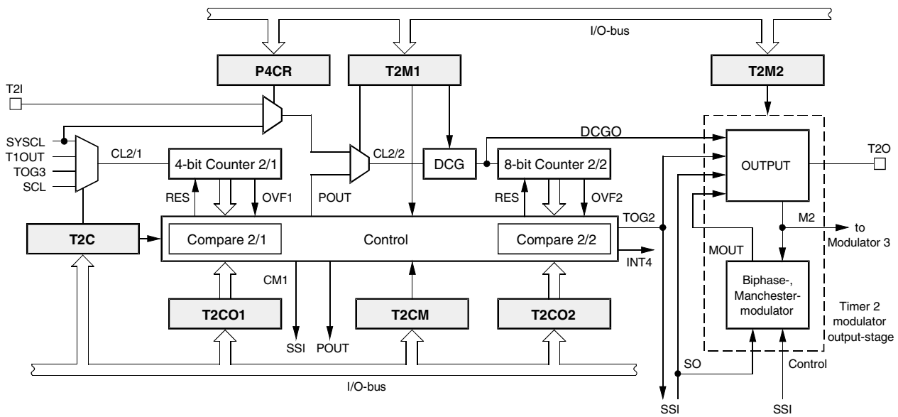
Figure 30. Timer 2
