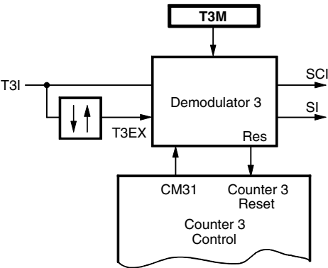
Figure 57. Timer 3 Demodulator 3
