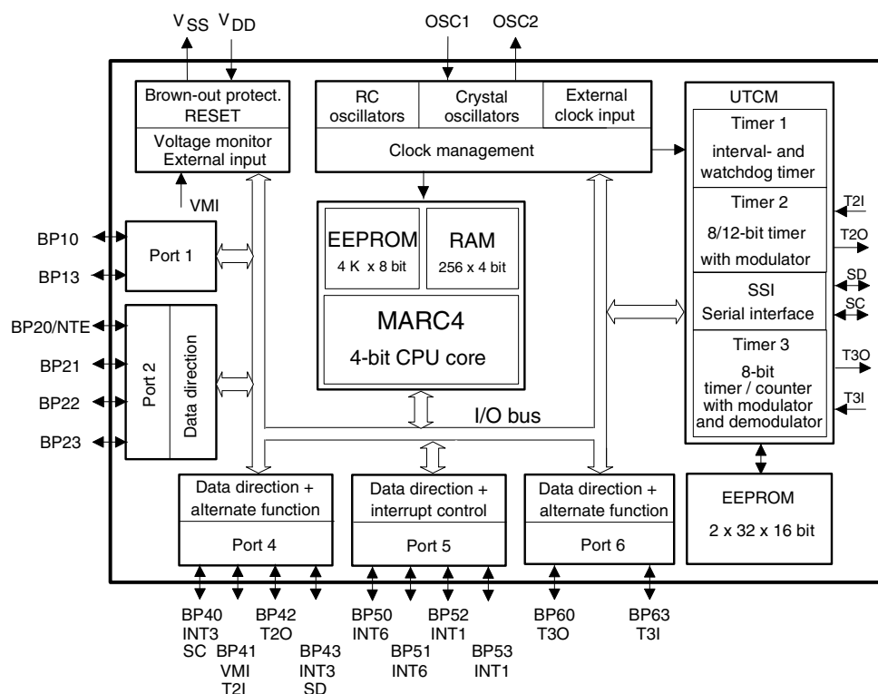
Figure 1. Block Diagram
