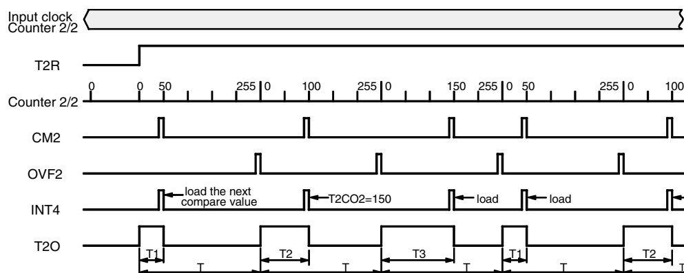
Figure 42. PWM Modulation
