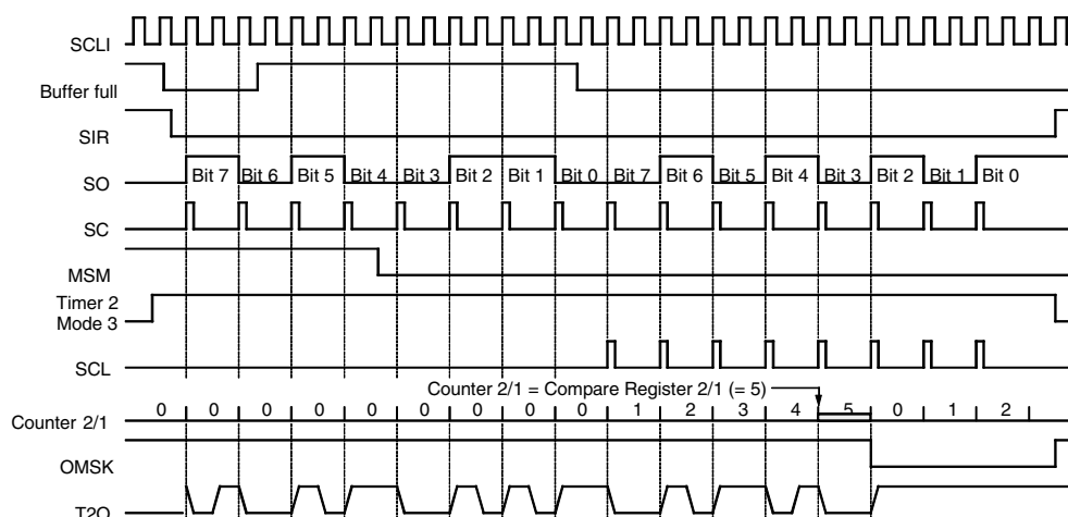
Figure 73. Bi-phase Modulation
