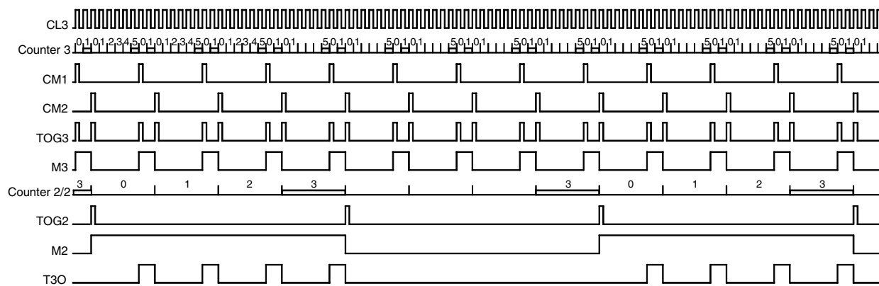
Figure 82. Burst Modulation 1
