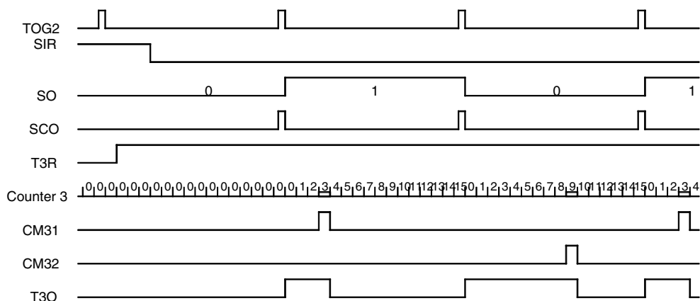
Figure 76. Pulse-width Modulation
