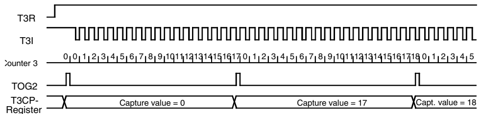
Figure 80. Frequency Measurement
