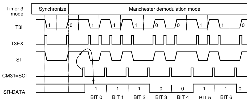
Figure 53. Manchester Demodulation
