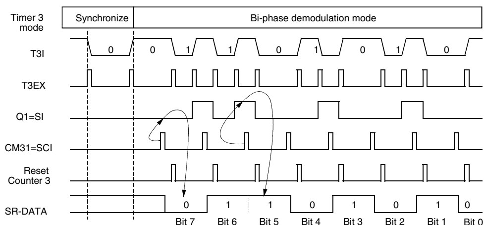
Figure 78. Bi-phase Demodulation
