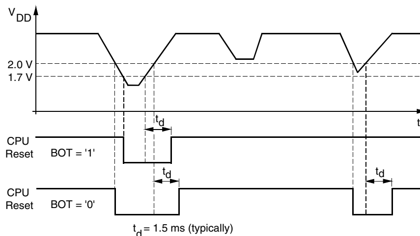
Figure 10. Brown-out Detection
