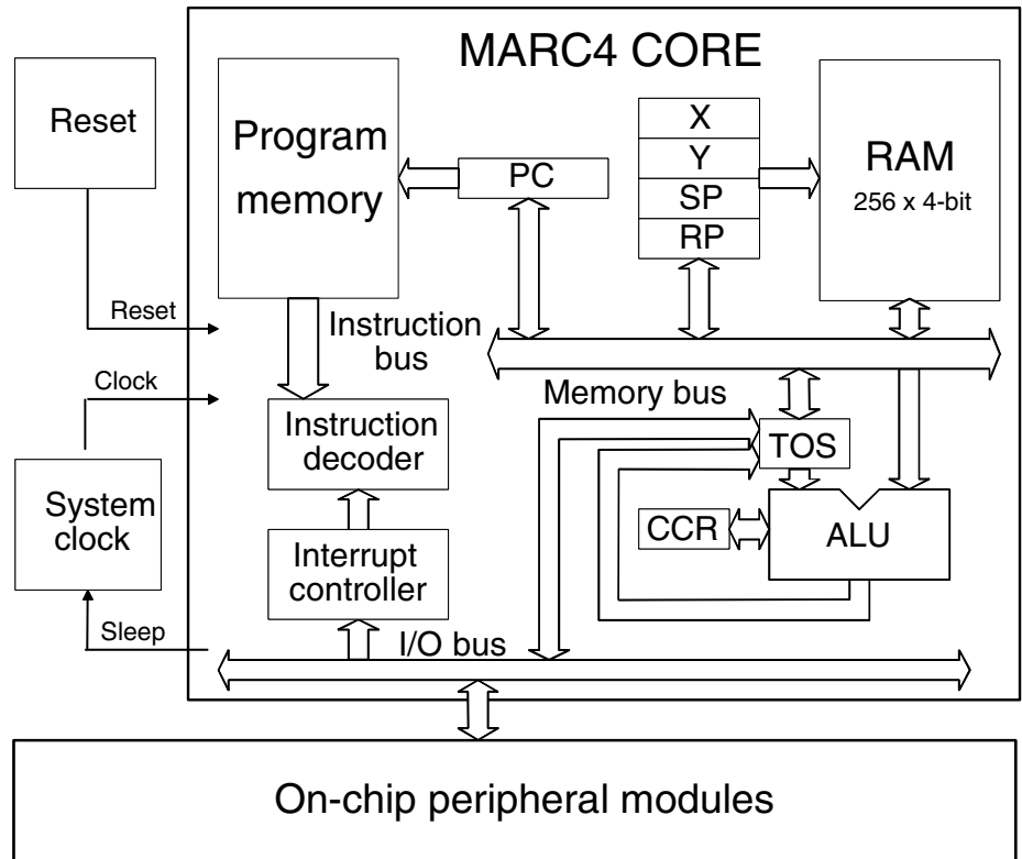
Figure 3. MARC4 Core
