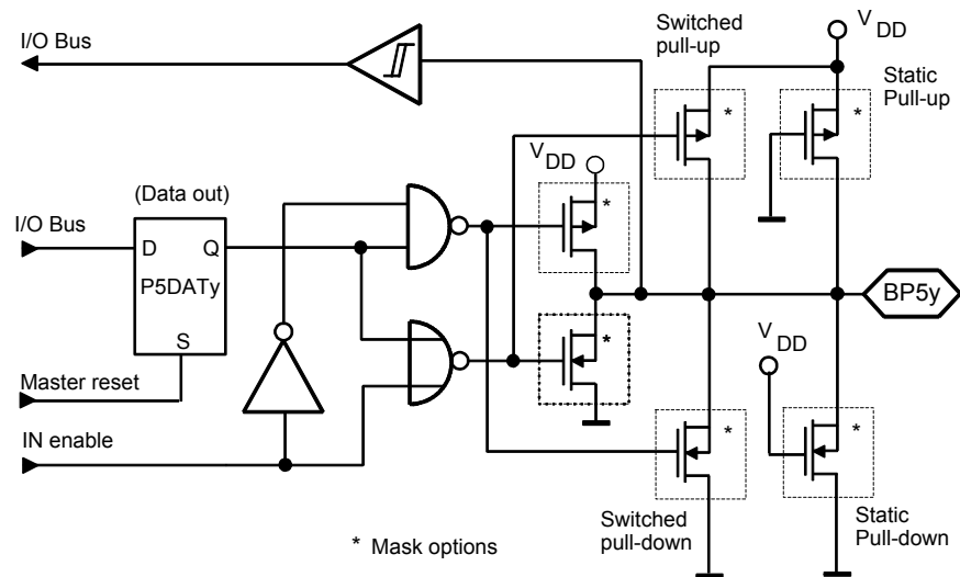
Figure 24. Bi-directional Port 5
