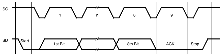
Figure 65. MCL Bus Protocol 2
