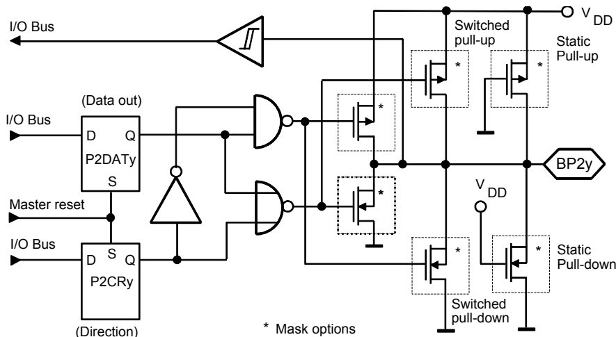
Figure 23. Bi-directional Port 2
