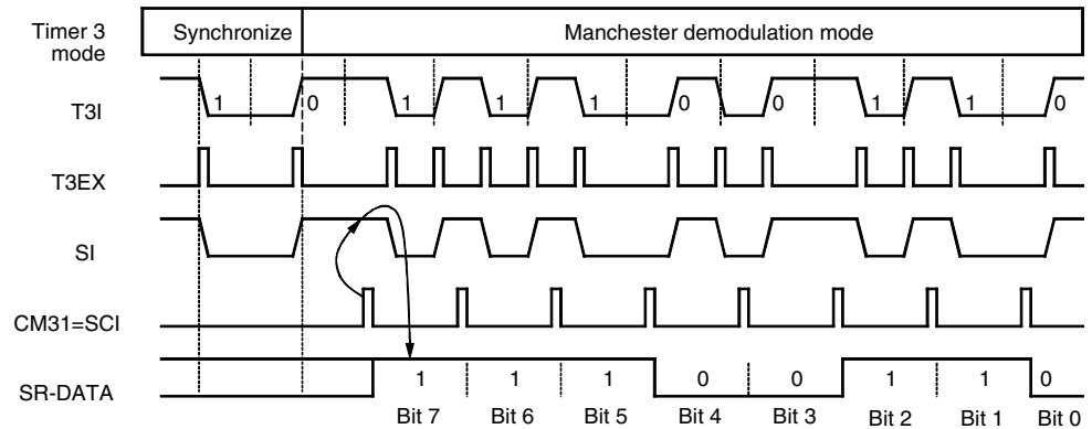
Figure 77. Manchester Demodulation
