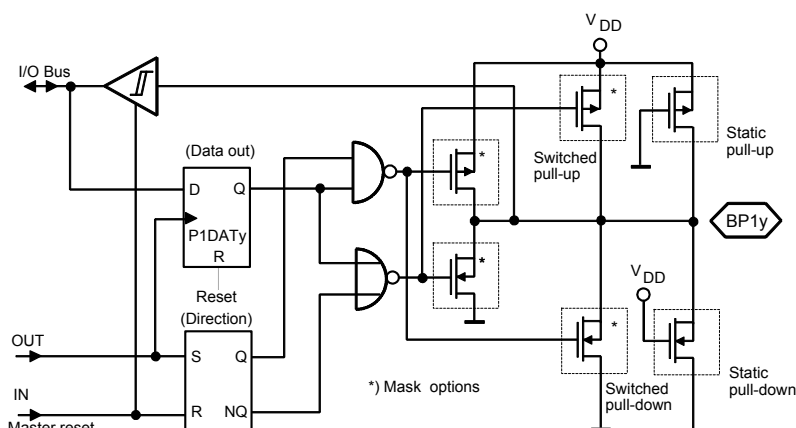
Figure 22. Bi-directional Port 1
