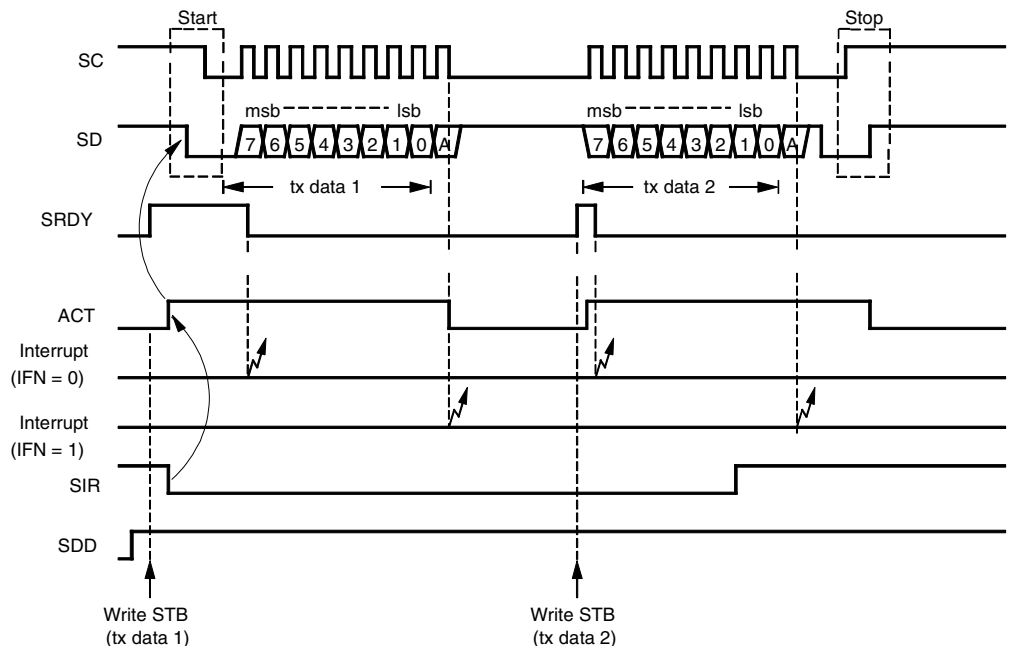
Figure 62. Example of MCL Transmit Dialog
