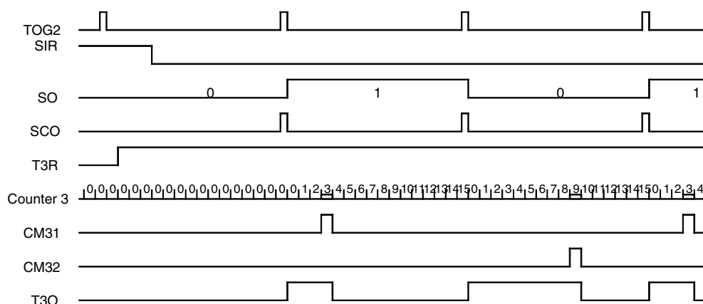
Figure 52. Pulse-width Modulation
