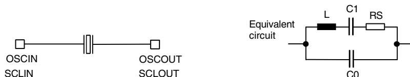
Figure 88. Crystal Equivalent Circuit
