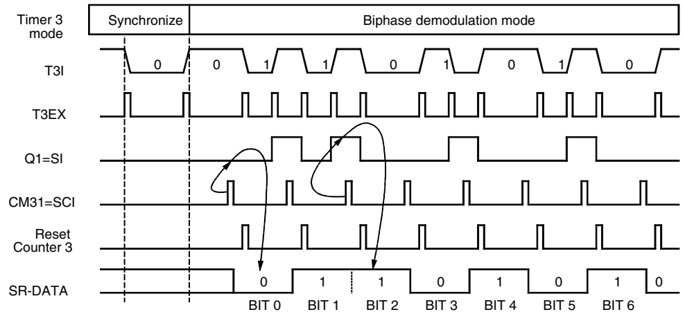
Figure 54. Bi-phase Demodulation
