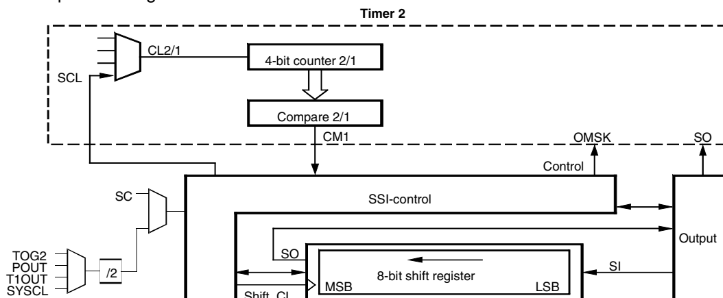
Figure 67. SSI Output Masking Function
