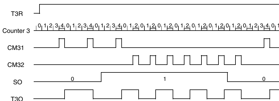
Figure 75. FSK Modulation
