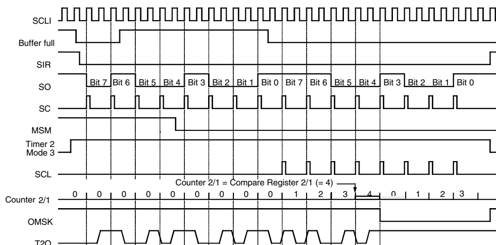
Figure 72. Manchester Modulation 2
