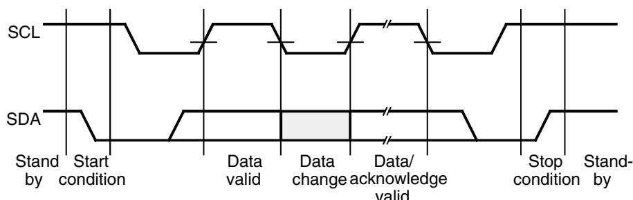
Figure 87. MCL Protocol
