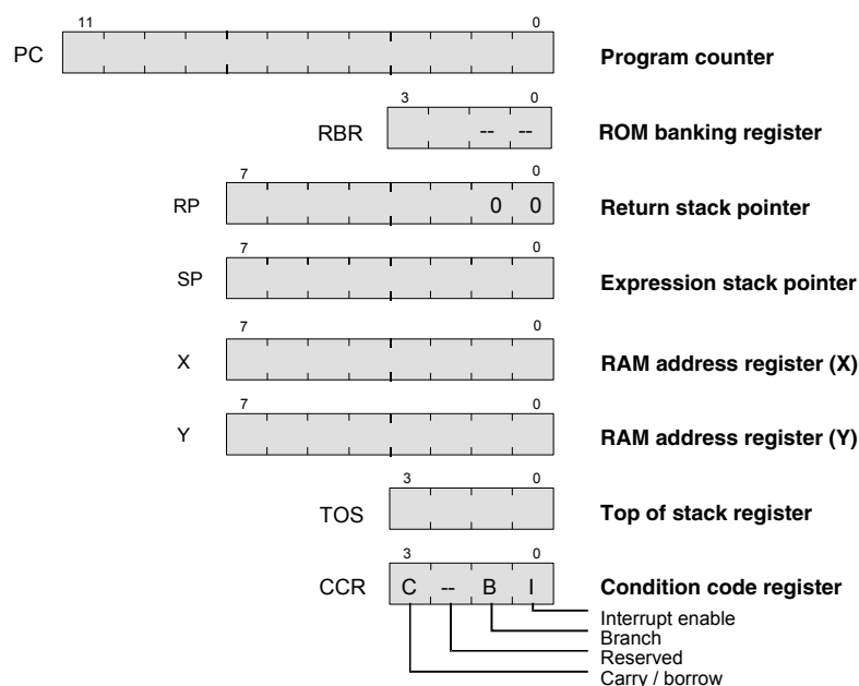
Figure 6. Programming Model
