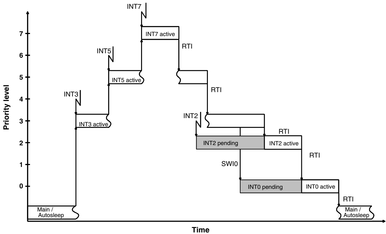
Figure 8. Interrupt Handling
