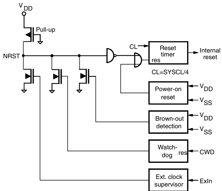
Figure 9. Reset Configuration
