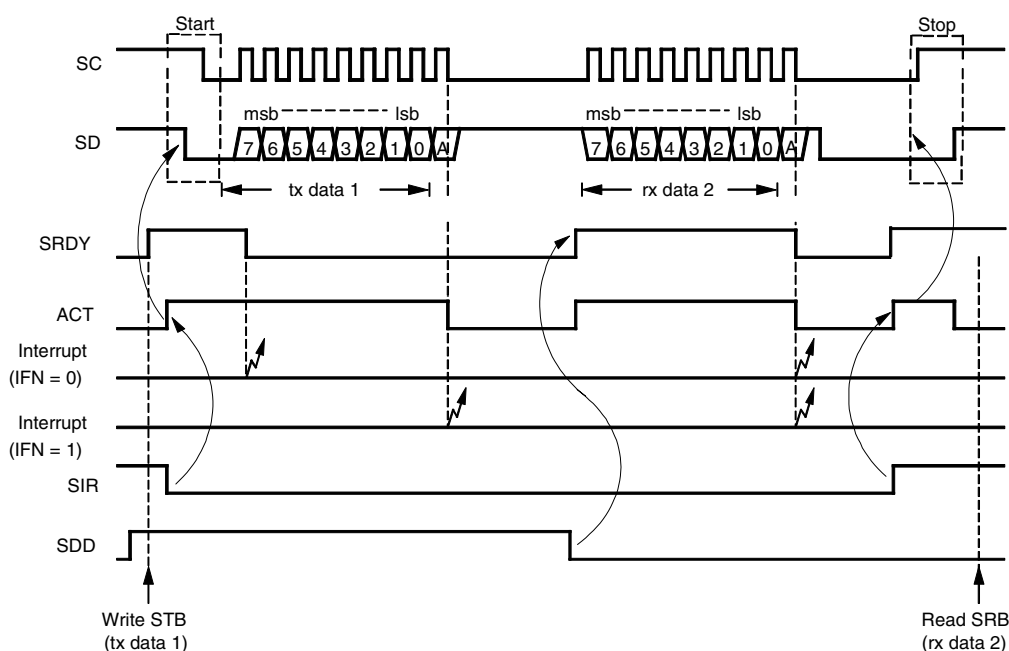
Figure 63. Example of MCL Receive Dialog
