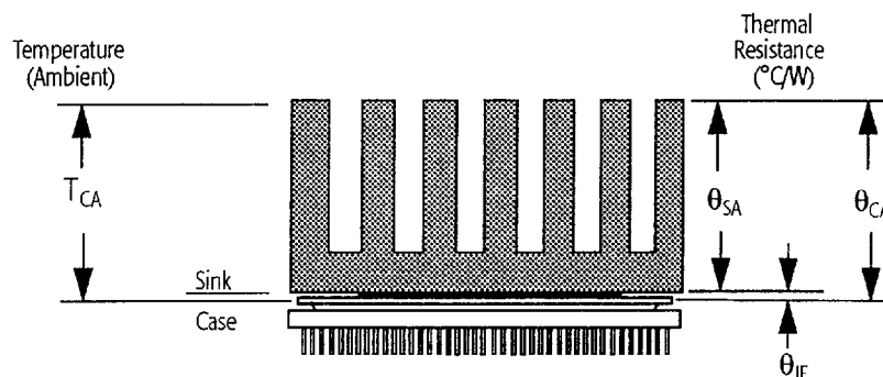
Figure 110. Thermal Model
