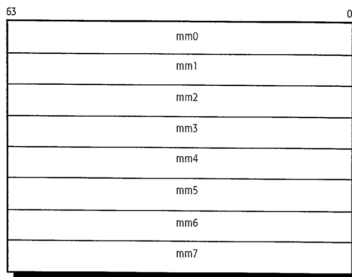
Figure 17. MMX™/3DNow!™ Registers
