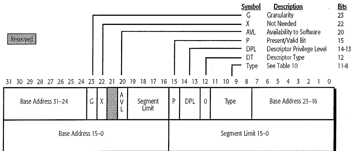
Figure 51. System Segment Descriptor
