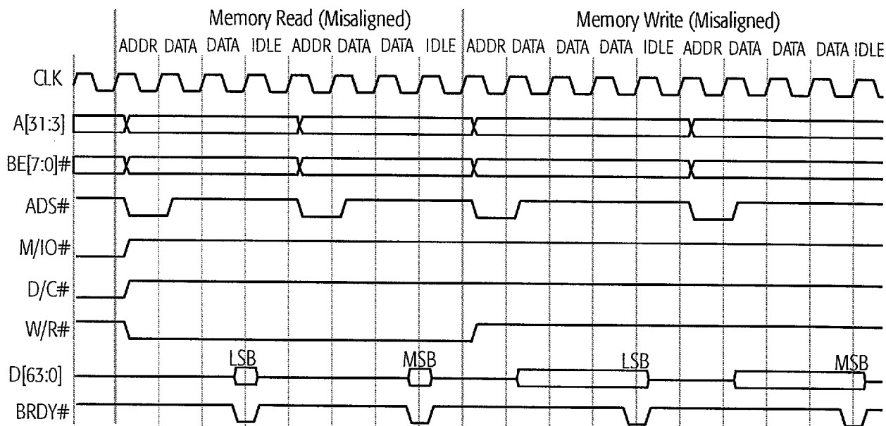
Figure 57. Misaligned Single-Transfer Memory Read and Write
