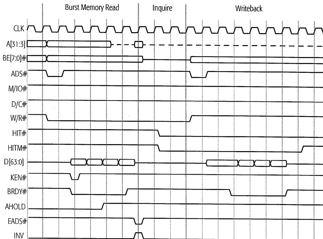
Figure 67. AHOLD-Initiated Inquire Hit to Modified Line
