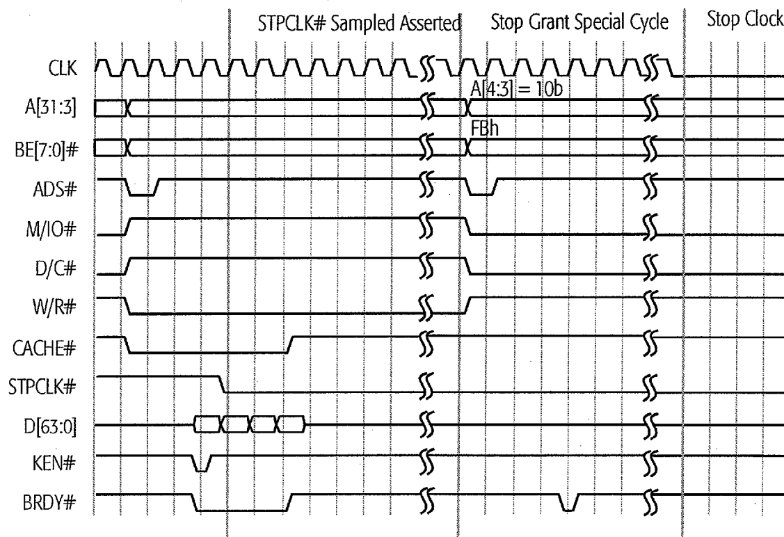
Figure 75. Stop Grant and Stop Clock Modes, Part 1
