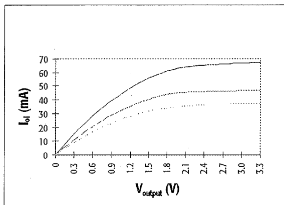
Figure 99. Pulldown V/I Curves
