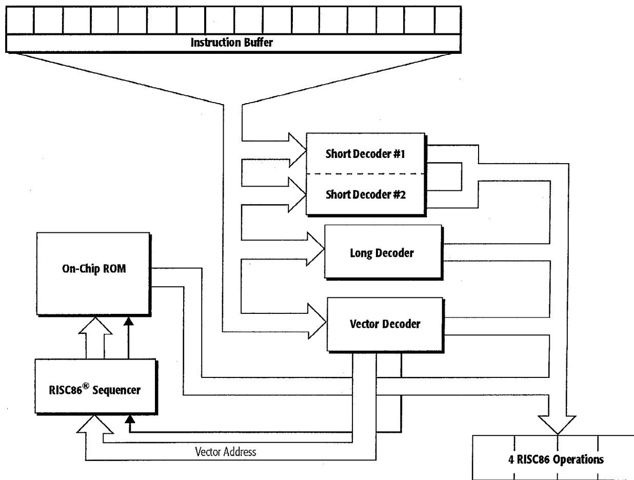
Figure 4. AMD-K6 ® -III Processor Decode Logic
