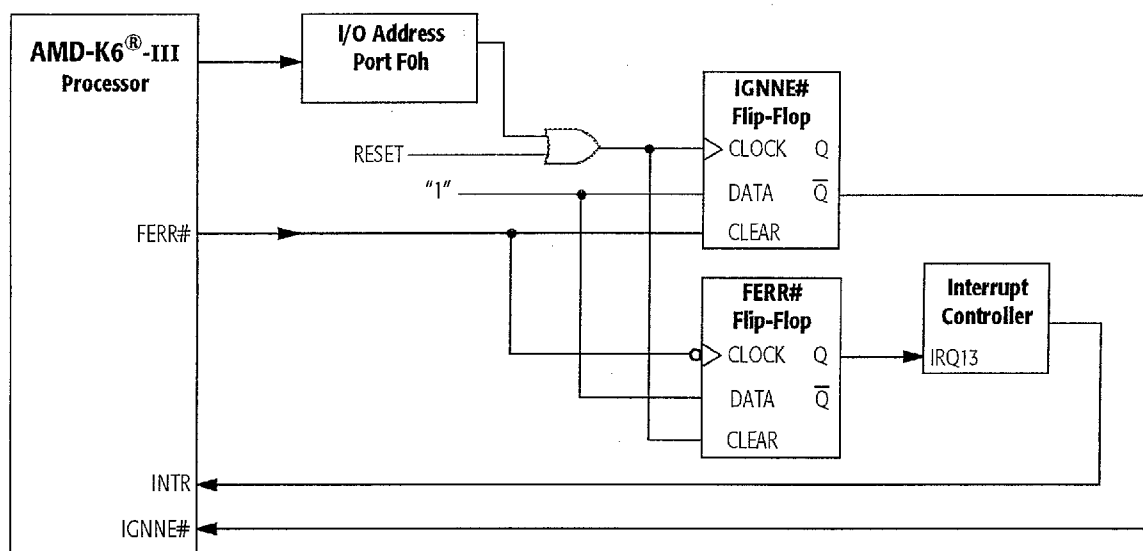
Figure 84. External Logic for Supporting Floating-Point Exceptions
