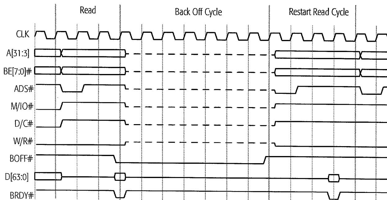
Figure 69. BOFF# Timing
