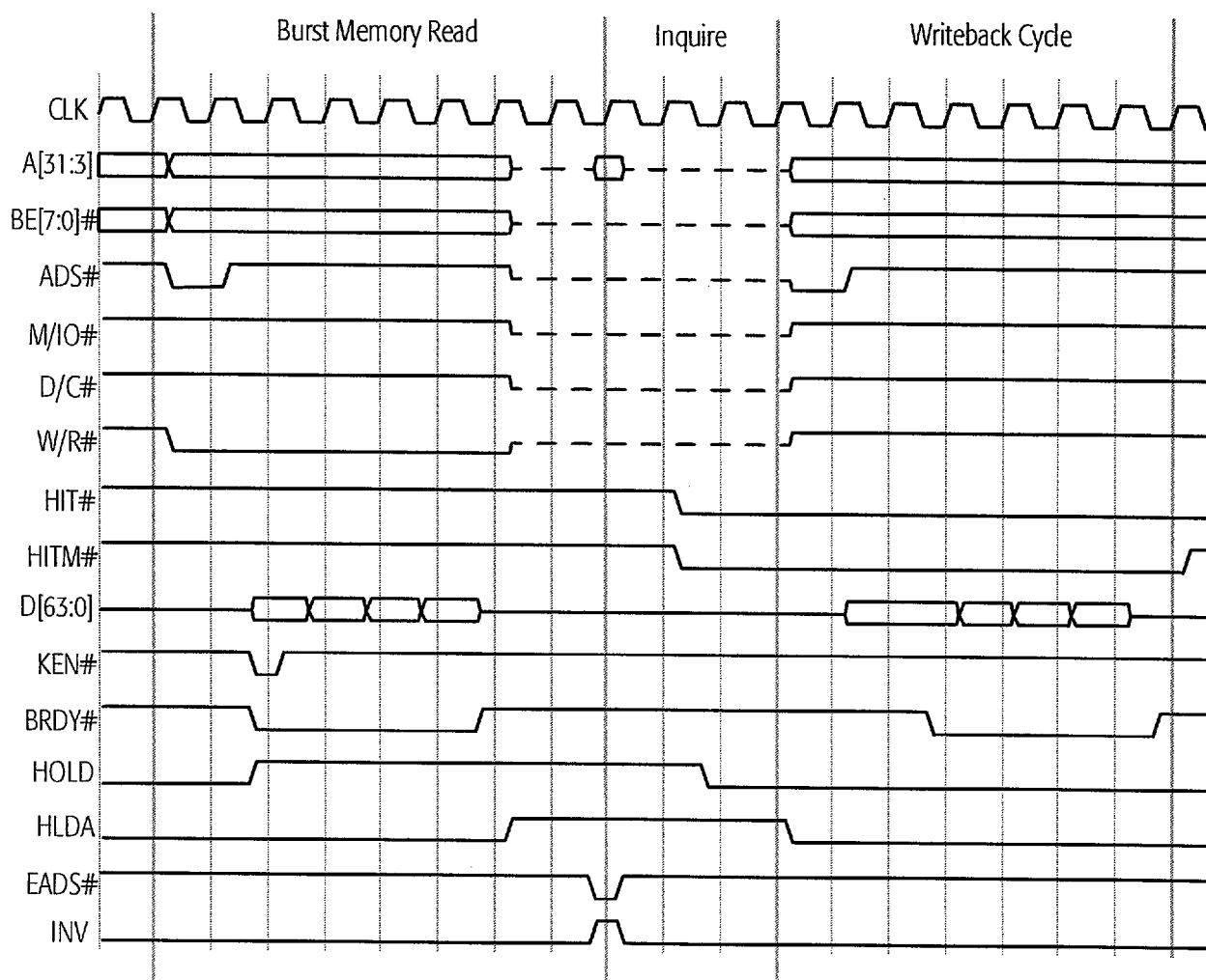
Figure 64. HOLD-Initiated Inquire Hit to Modified Line
