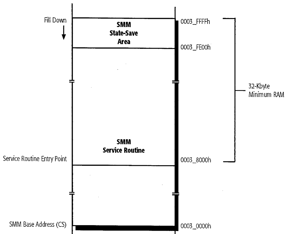
Figure 85. SMM Memory
