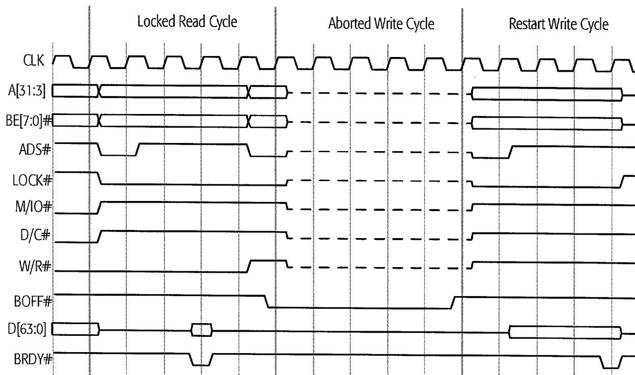
Figure 71. Locked Operation with BOFF# Intervention
