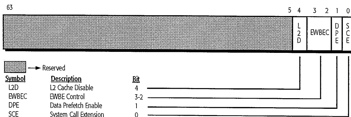
Figure 34. Extended Feature Enable Register (EFER)—MSR C000_0080h
