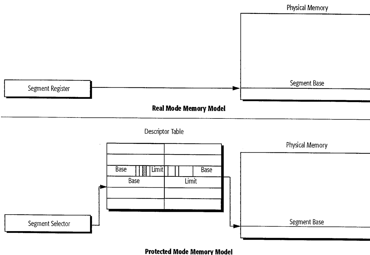
Figure 10. Segment Usage
