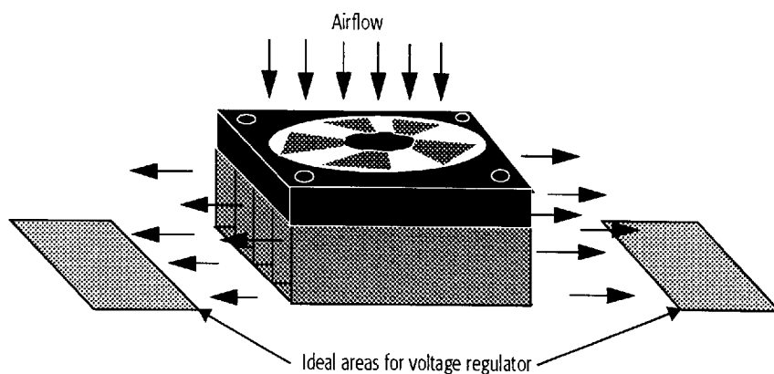
Figure 115. Airflow for a Heatsink with Fan
