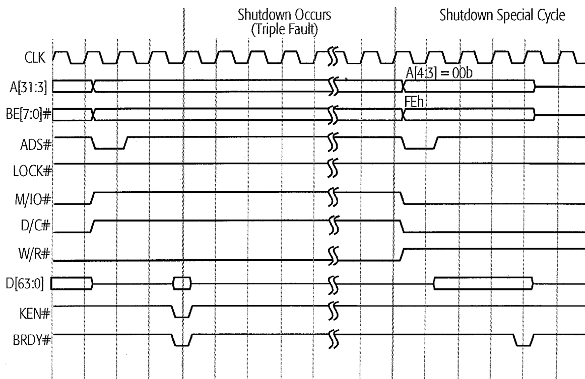
Figure 74. Shutdown Cycle
