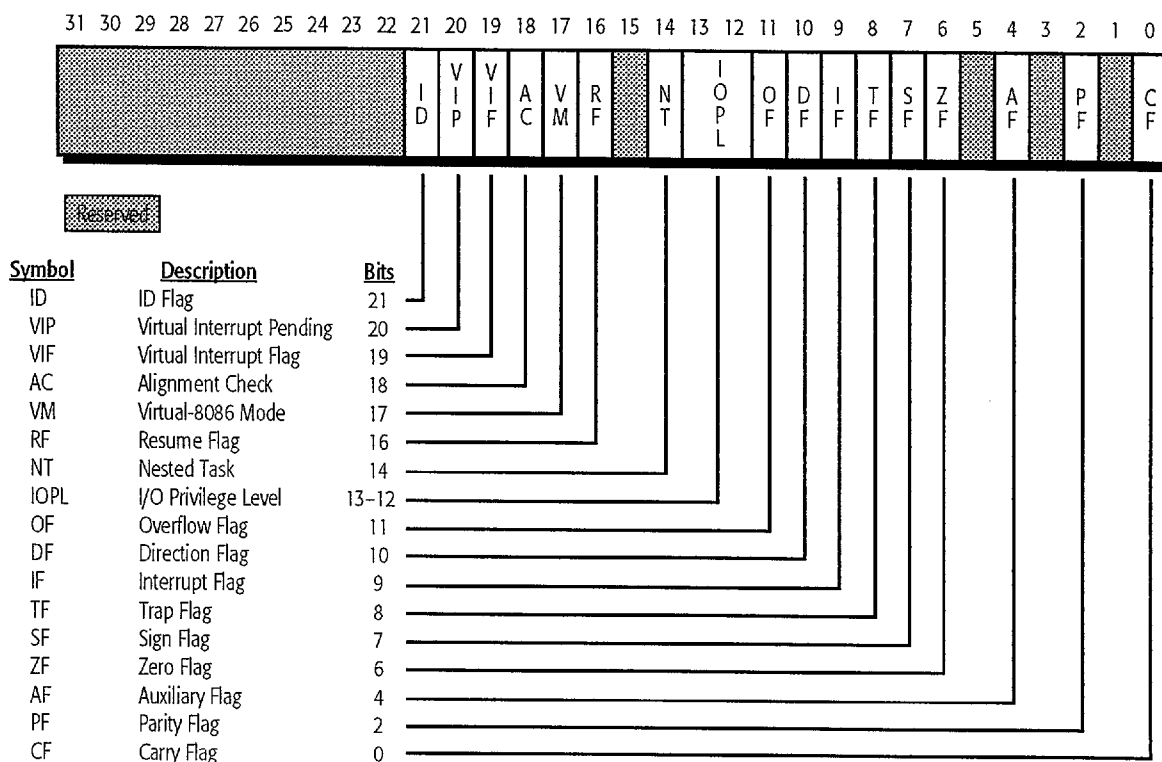
Figure 20. EFLAGS Registers
