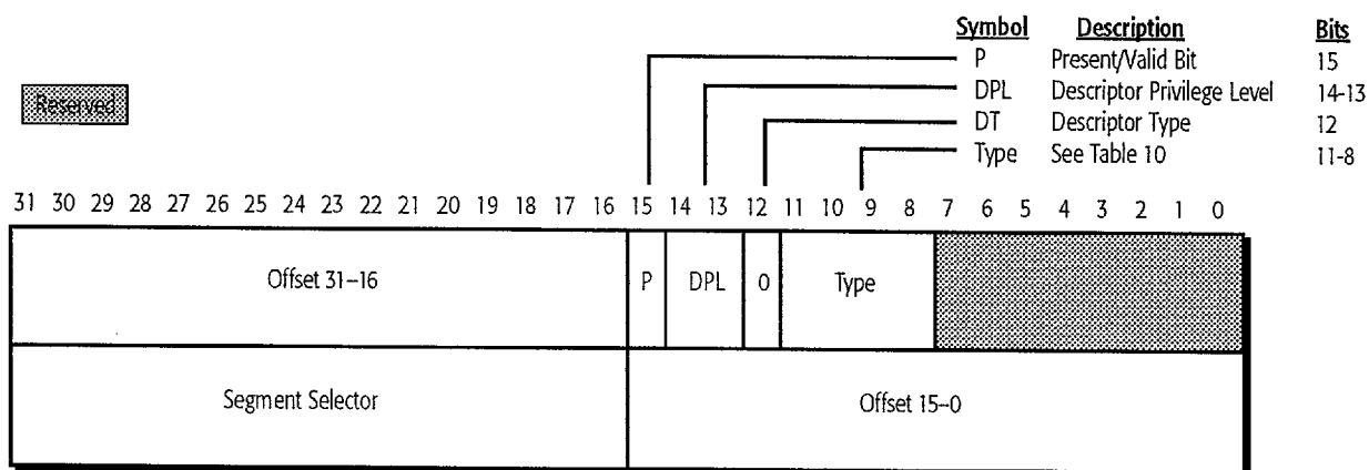
Figure 52. Gate Descriptor
