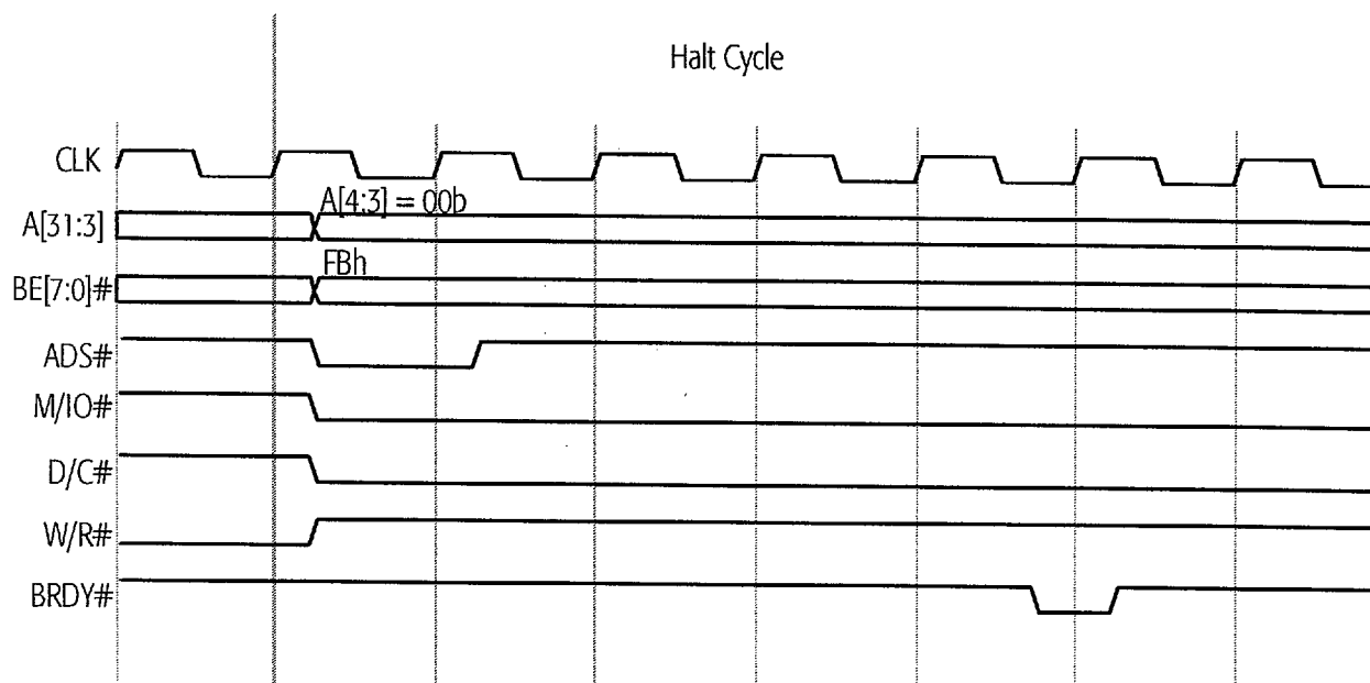
Figure 73. Basic Special Bus Cycle (Halt Cycle)
