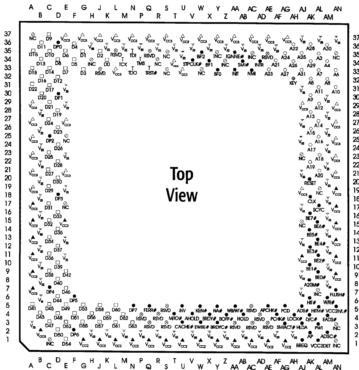
Figure 118. AMD-K6®-III Processor Top-Side View
