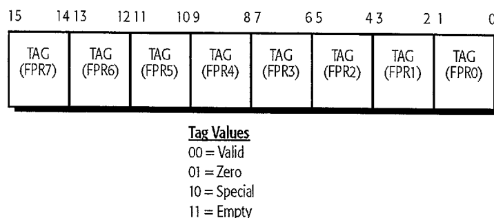
Figure 14. FPU Tag Word Register
