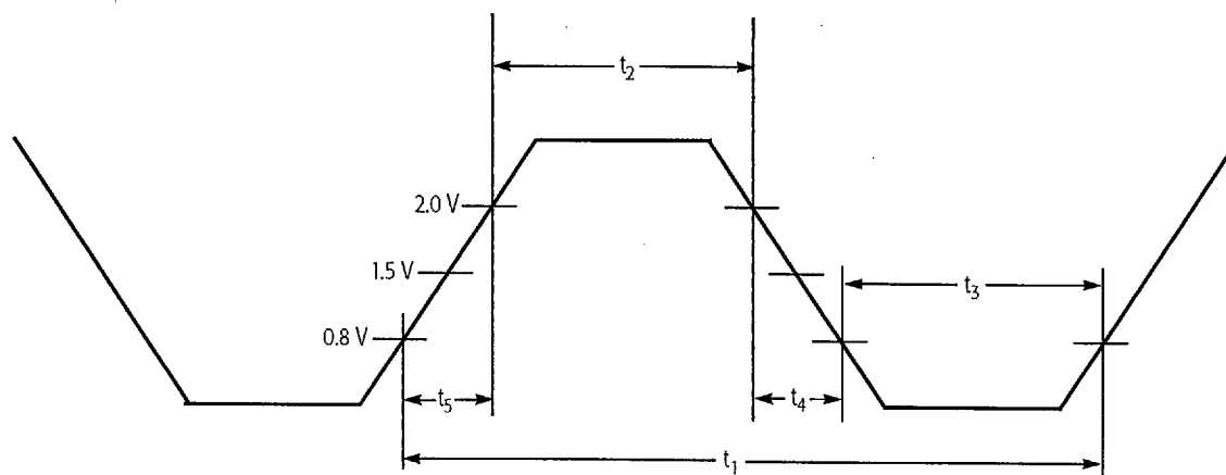
Figure 101. CLK Waveform
