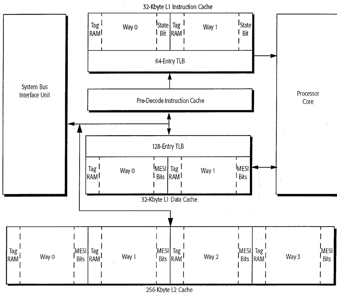
Figure 78. L1 and L2 Cache Organization
