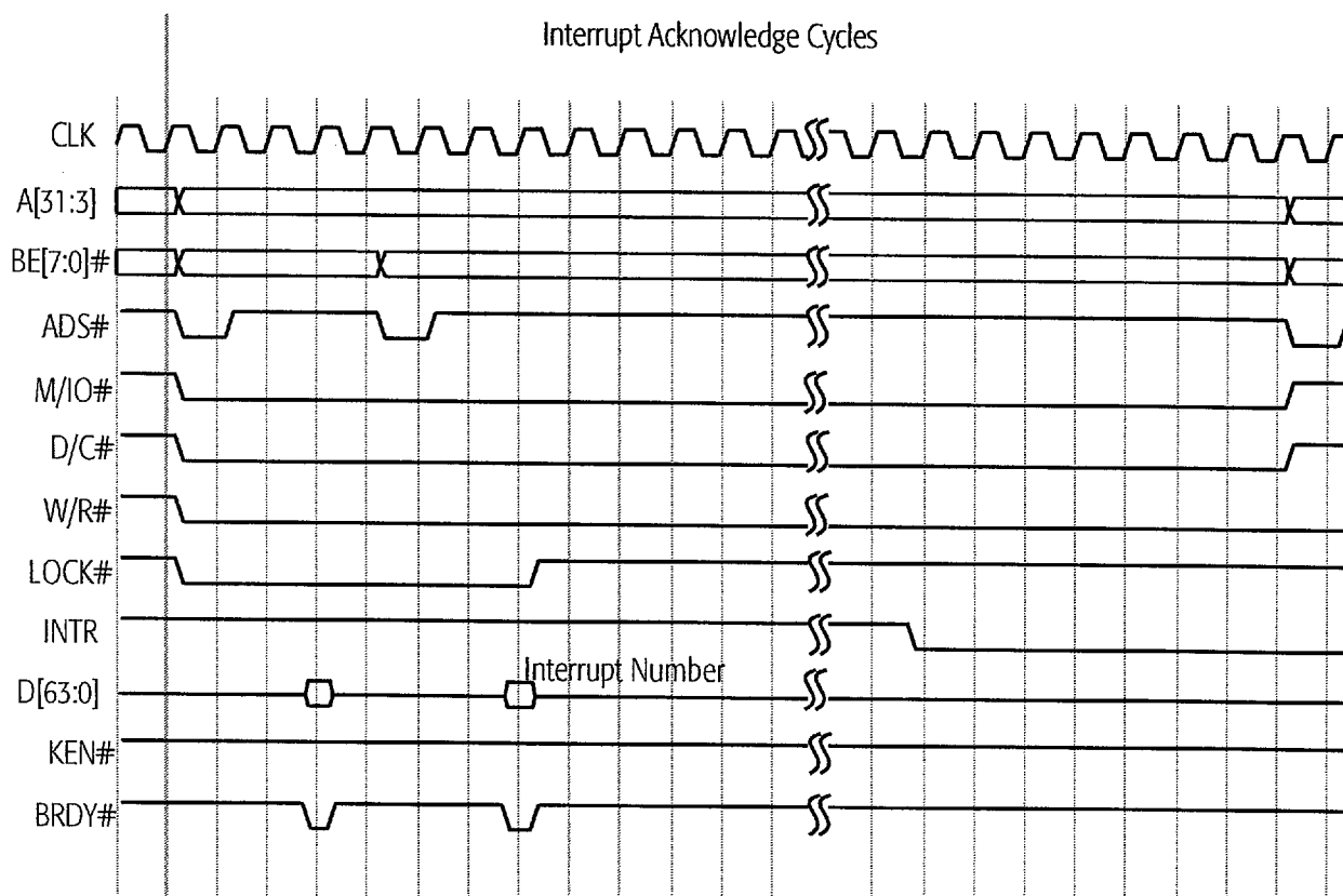
Figure 72. Interrupt Acknowledge Operation
