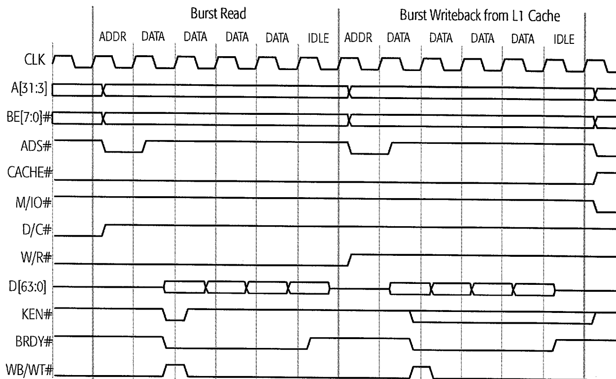
Figure 59. Burst Writeback due to Cache-Line Replacement
