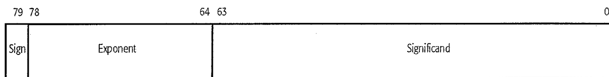
Figure 11. Floating-Point Register
