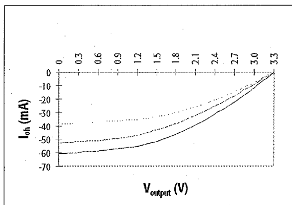
Figure 100. Pullup V/I Curves
