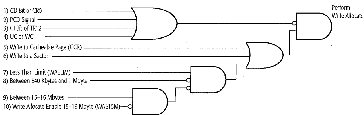
Figure 81. Write Allocate Logic Mechanisms and Conditions
