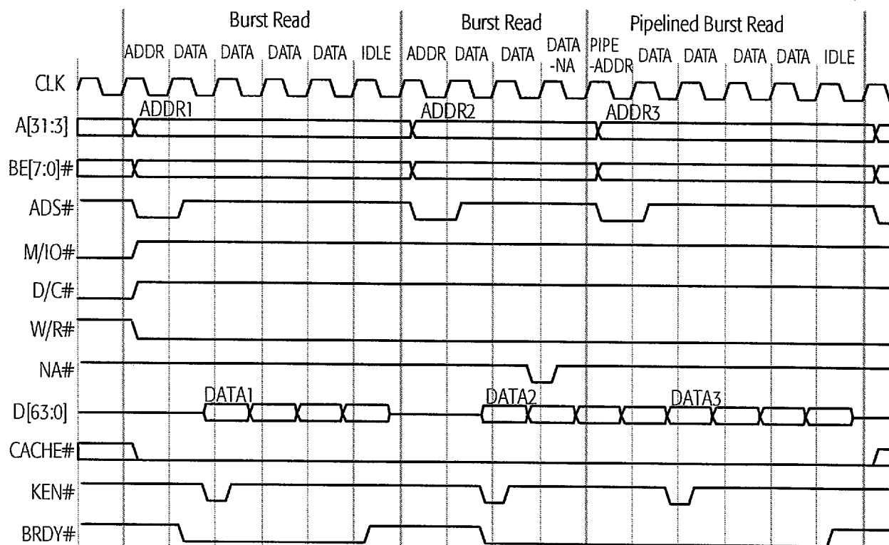
Figure 58. Burst Reads and Pipelined Burst Reads
