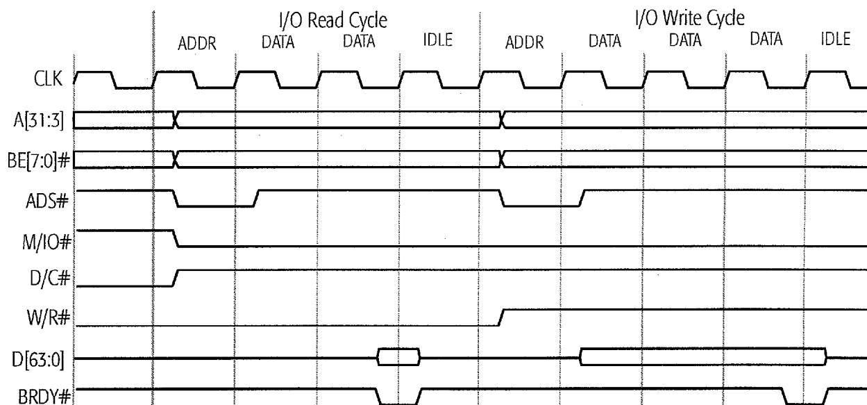
Figure 60. Basic I/O Read and Write
