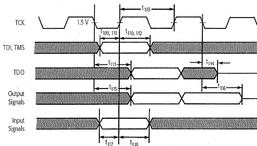
Figure 109. Test Signal Timing Diagram
