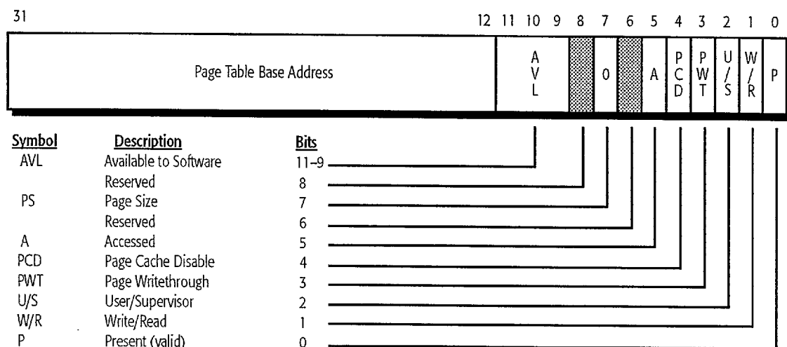
Figure 47. Page Directory Entry 4-Kbyte Page Table (PDE)
