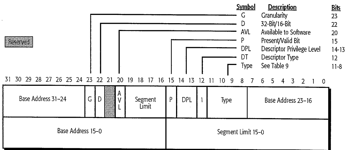
Figure 50. Application Segment Descriptor
