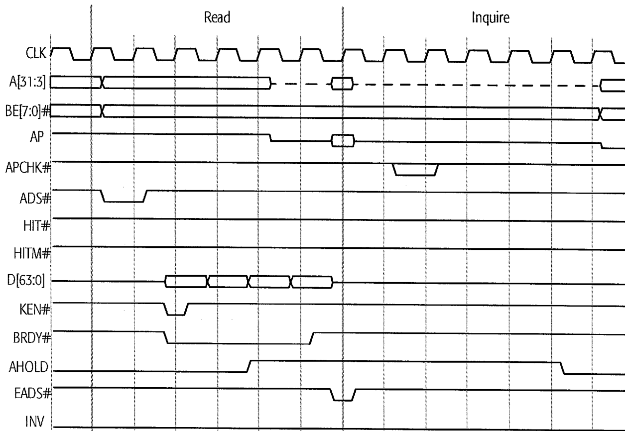
Figure 65. AHOLD-Initiated Inquire Miss
