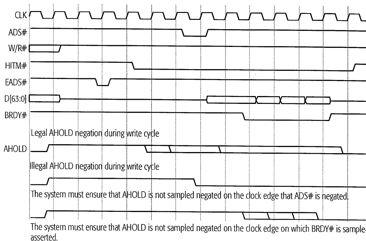
Figure 68. AHOLD Restriction
