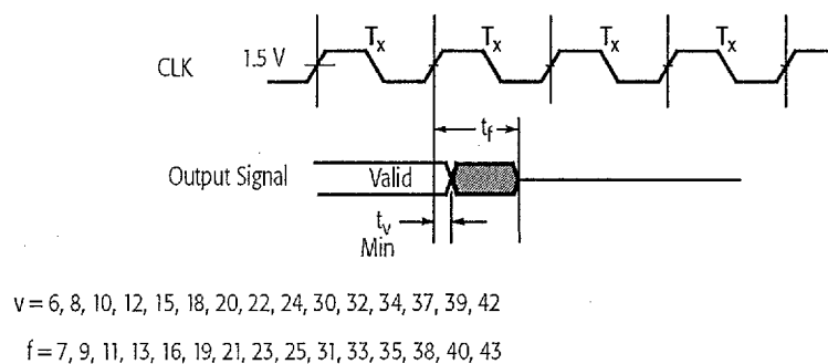
Figure 104. Maximum Float Delay Timing
