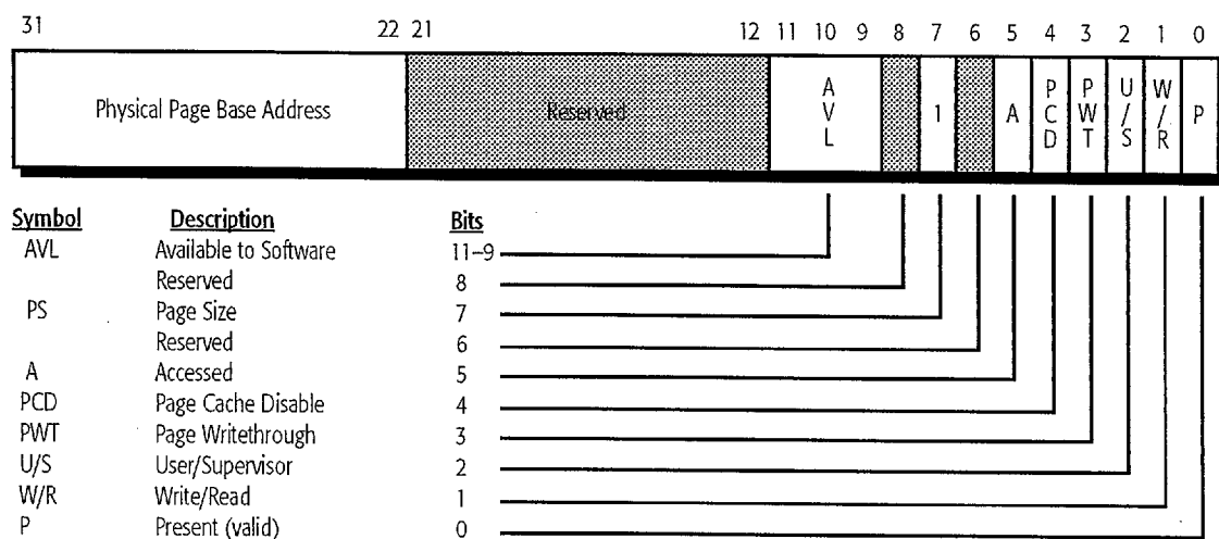
Figure 48. Page Directory Entry 4-Mbyte Page Table (PDE)
