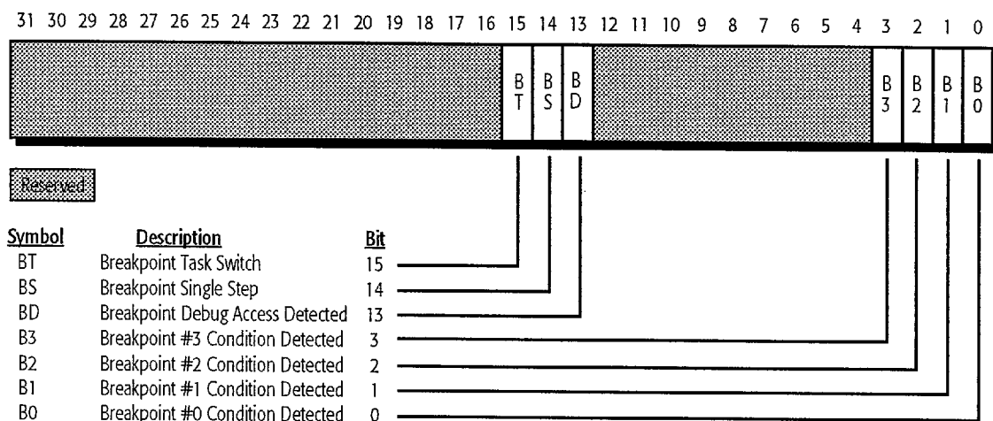
Figure 27. Debug Register DR6
