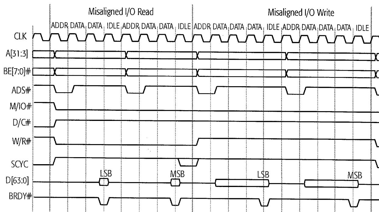
Figure 61. Misaligned I/O Transfer
