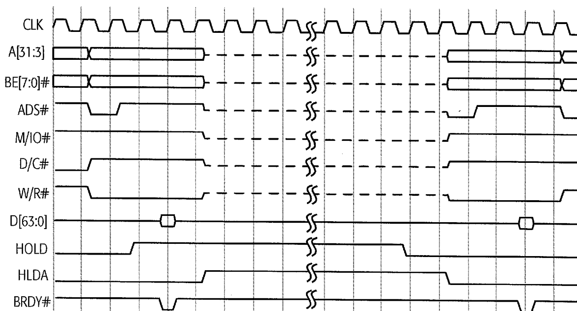
Figure 62. Basic HOLD/HLDA Operation
