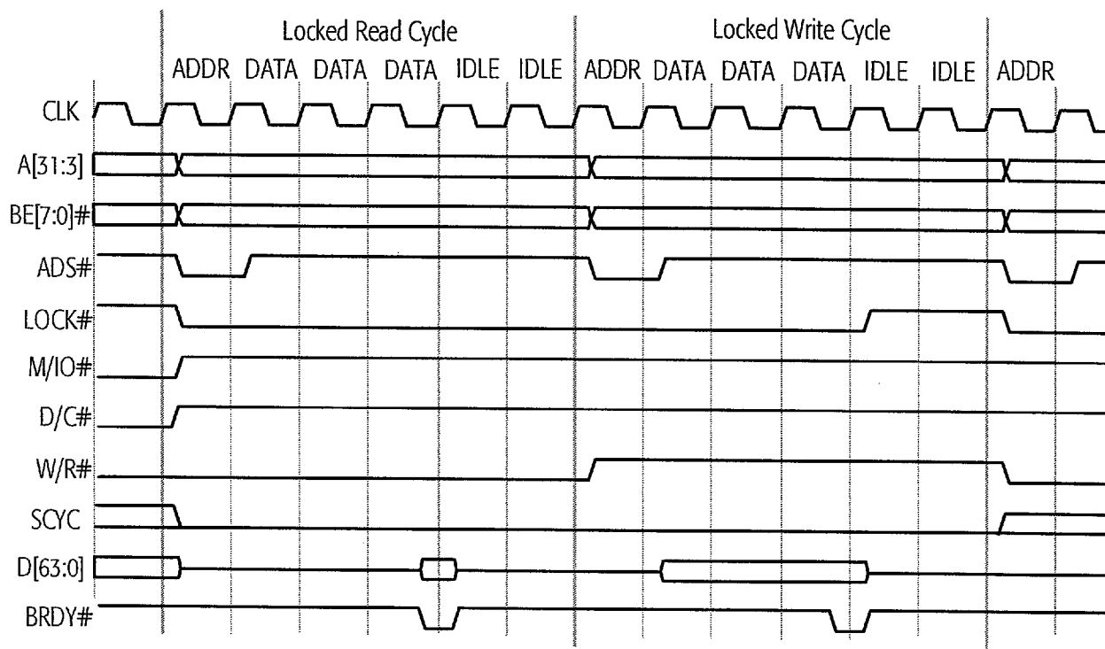
Figure 70. Basic Locked Operation
