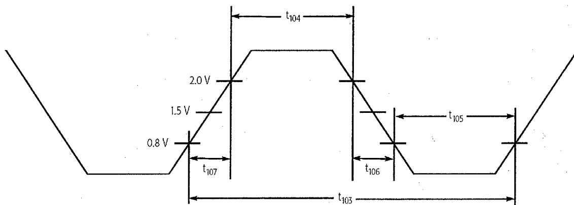
Figure 107. TCK Waveform
