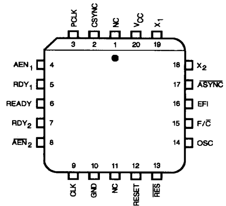
PLCC
