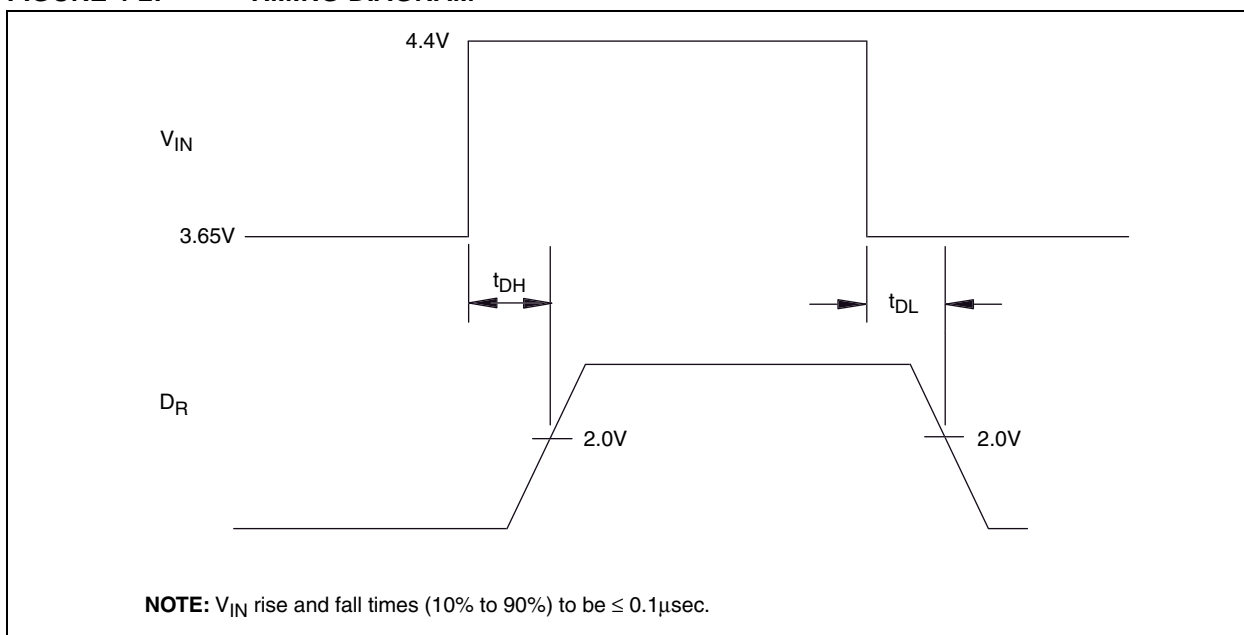
FIGURE 4-2: TIMING DIAGRAM
