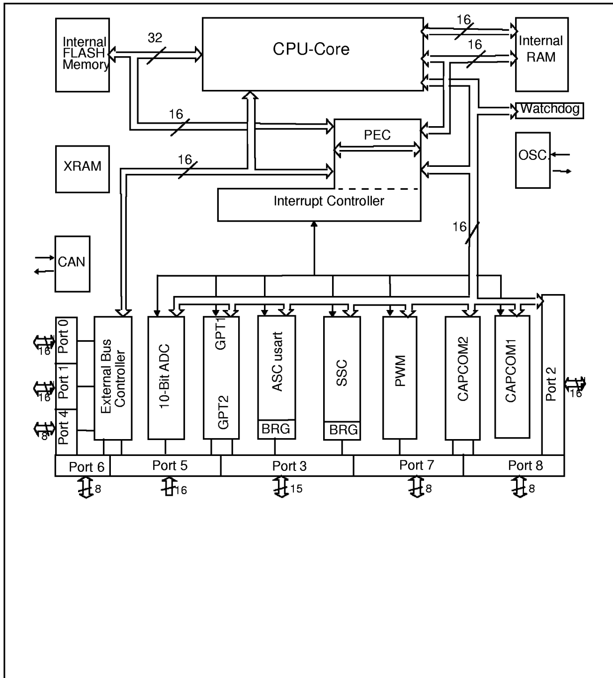
Figure 3 : Block diagram
