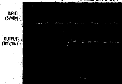
MAX527 NEGATIVE SETTLING TIME TO FULL-SCALE STEP—ALL BITS ON TO ALL BITS OFF
