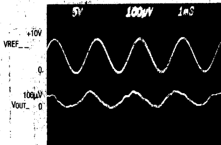
1ms/div TOP: REFERENCE IN 5V/div BOTTOM: VOUT 100µV/div INPUT CODE = ALL 0s
