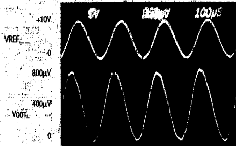
100µs/div TOP: REFERENCE IN 5V/div BOTTOM: VOUT 200µV/div INPUT CODE = ALL 0s
