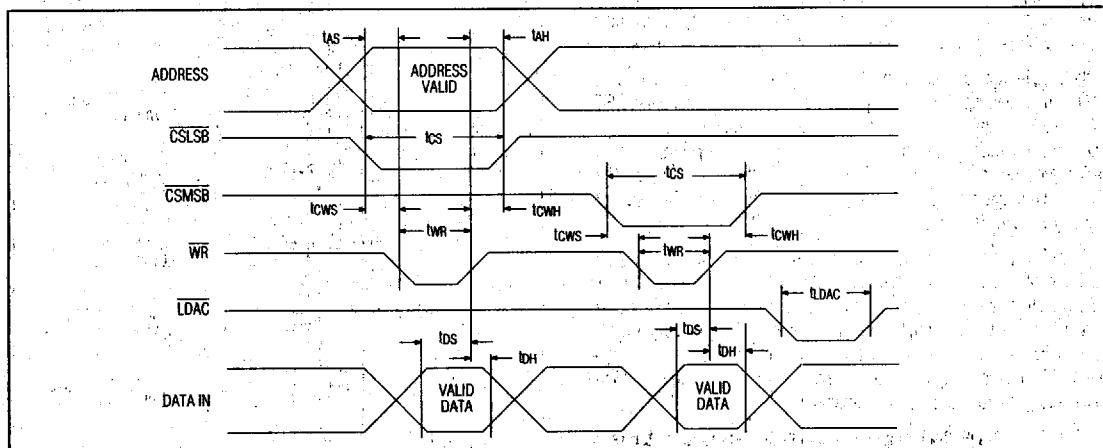
Figure 3. Write-Cycle Timing
