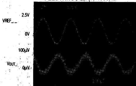
MAX527 REFERENCE FEEDTHROUGH AT 4000Hz
