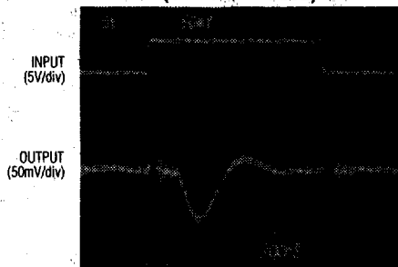
MAX527 DIGITAL FEEDTHROUGH (GLITCH IMPULSE)
