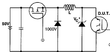
Fig. 13a - Clamped Inductive Load Test Circuit
