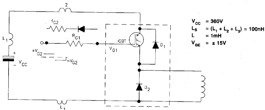
Fig. 16 - Test Circuit for Measurement of I_{LM} , E_{ON} , E_{OFF} , Q_{RR} , I_{RR} , t_{D(ON)} , t_r , t_{D(OFF)} , t
