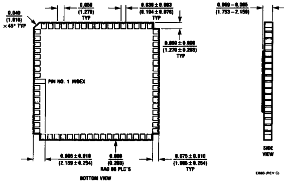
Leadless Chip Carrier (E) Order Number HPC16164E NS Package Number E68B
