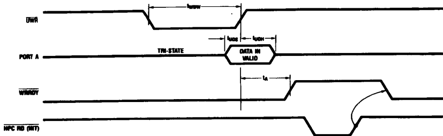
FIGURE 7. UPI Write Timing
