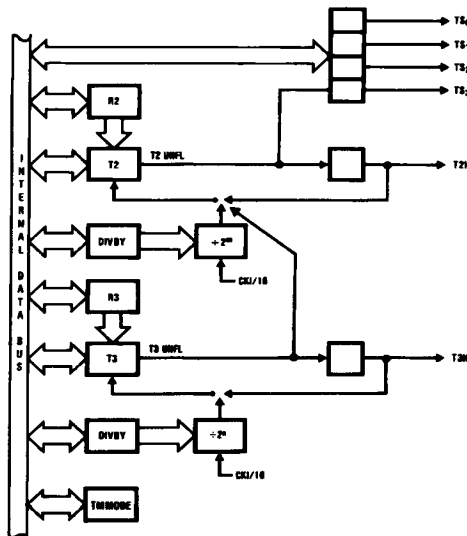
FIGURE 16. Timers T2-T3 Block
