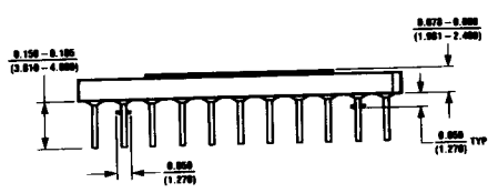
Pin Grid Array Package (U) Order Number HPC16164U NS Package Number U68C
