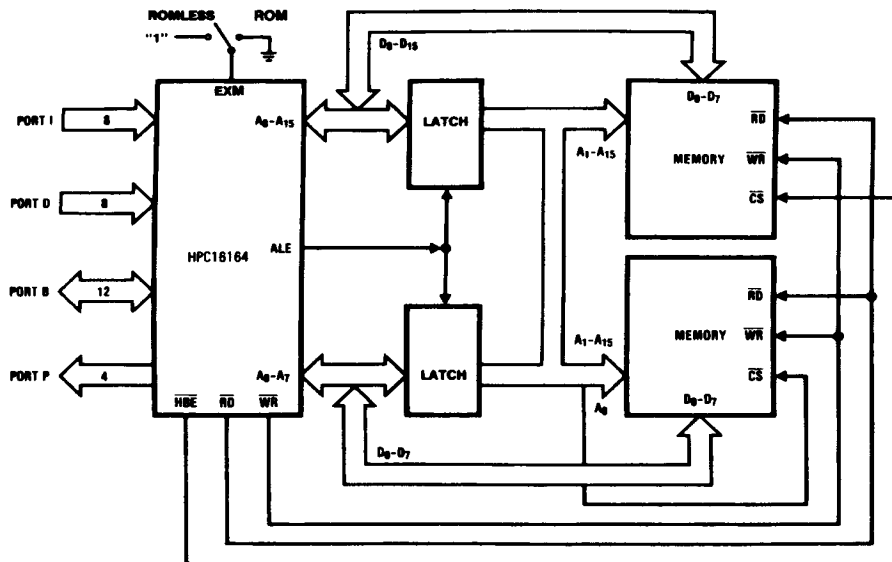
FIGURE 13. 16-Bit External Memory
