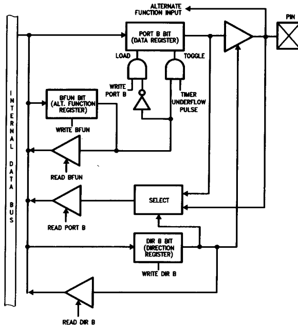
FIGURE 9. Structure of Port B Pins B3, B4, B8, B9, B13 and B14 (Timer Synchronous Pins)
