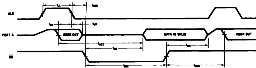
FIGURE 2. Read Cycle
