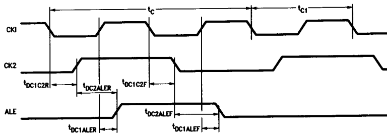
CK1, CK2, ALE Timing Diagram
