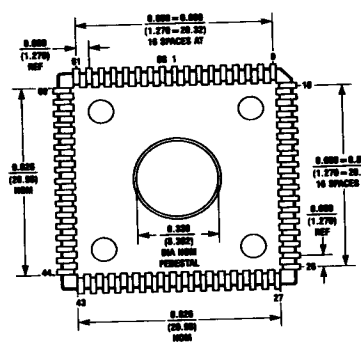
Plastic Leaded Chip Carrier (V) Order Number HPC16164V NS Package Number V68A
