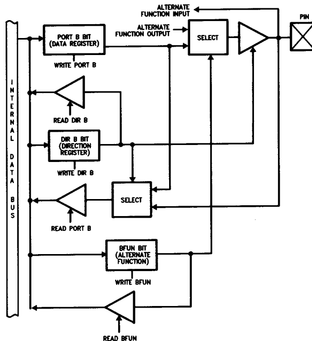
FIGURE 8. Structure of Port B Pins B0, B1, B2, B5, B6 and B7 (Typical Pins)
