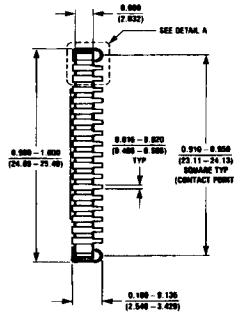
Leadless Chip Carrier (E) Order Number HPC16164E NS Package Number E68B
