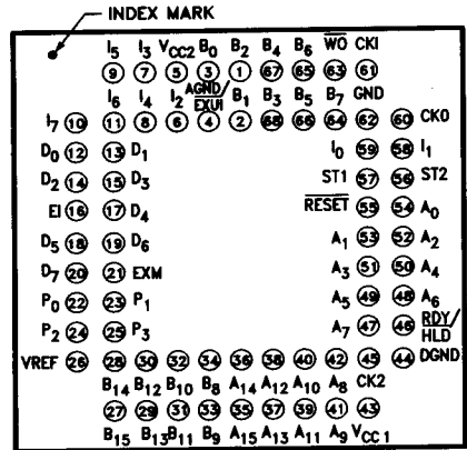
Top View (looking down on component side of PC Board)
