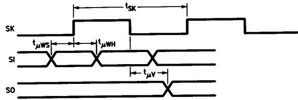
FIGURE 5. MICROWIRE Setup/Hold Timing
