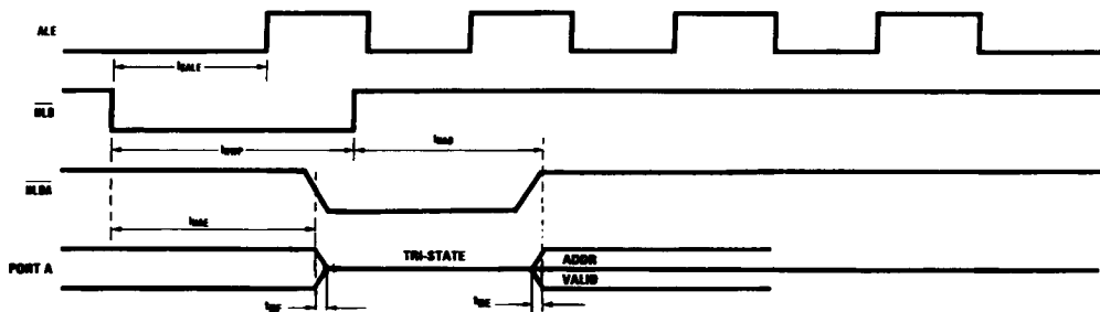
FIGURE 4. Hold Mode Timing
