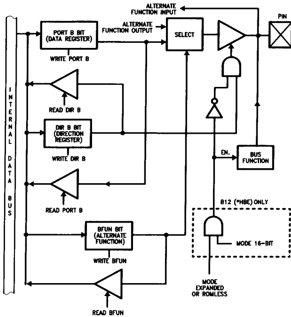
FIGURE 10. Structure of Port B Pins B10, B11, B12 and B15 (Pins with Bus Control Roles)
