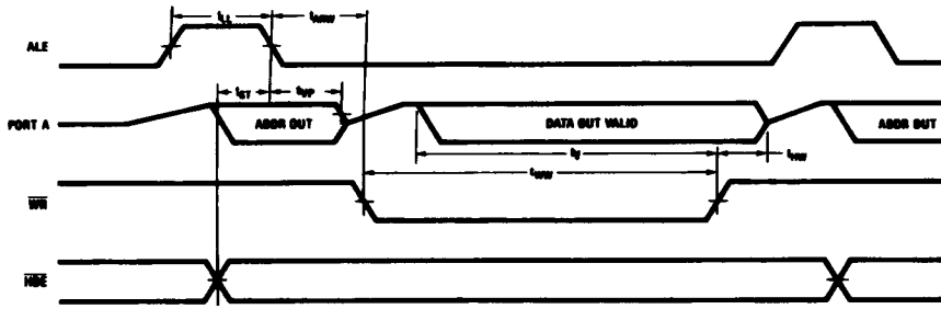
FIGURE 1. Write Cycle
