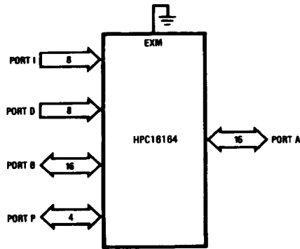
FIGURE 11. Single-Chip Mode
