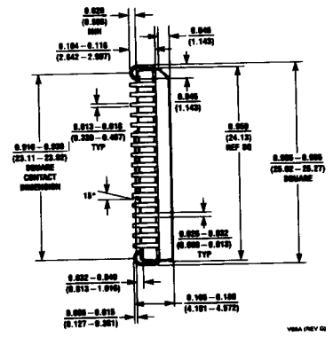
Plastic Leaded Chip Carrier (V) Order Number HPC16164V NS Package Number V68A
