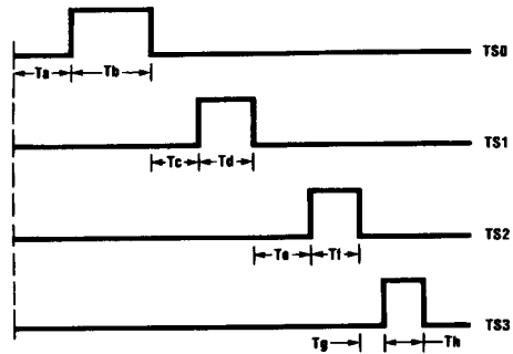
FIGURE 19. Synchronous Pulse Generation
