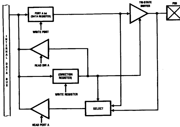
FIGURE 7. Port A: I/O Structure
