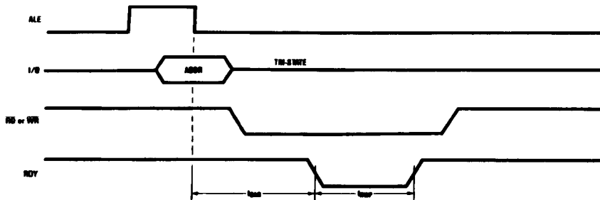
FIGURE 3. Ready Mode Timing
