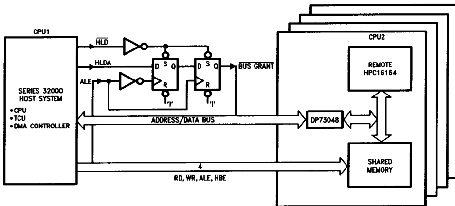
FIGURE 25. Shared Memory Application: HPC16164 Interface to Series 32000 System
