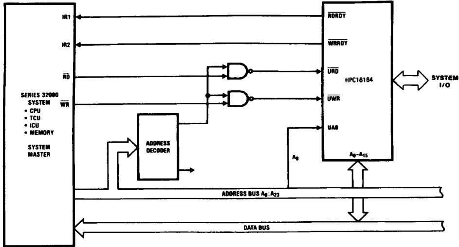
FIGURE 24. HPC16164 as a Peripheral: (UPI Interface to Series 32000 Application)
