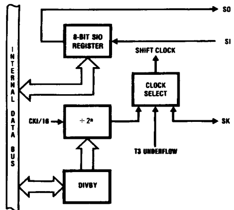
FIGURE 20. MICROWIRE/PLUS
