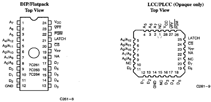
Figure 1. Programming Pinouts
