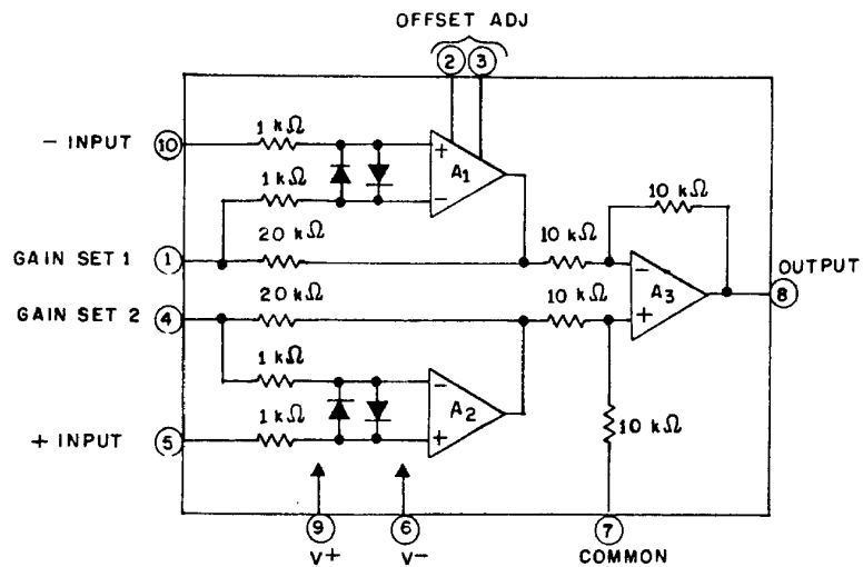
FIGURE 2. Block diagrams.
