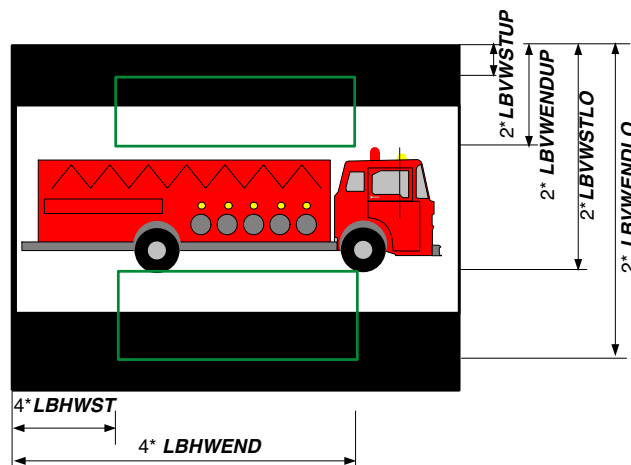
Fig. 2-28: Measurement Windows
