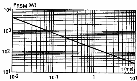
Fig. 4 - Non repetitive surge peak reverse power dissipation PRSM versus pulse duration at T_j initial = 25^\circ\text{C} (maximum values).
