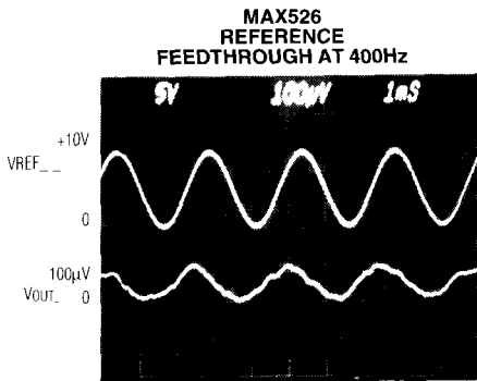
1ms/div TOP: REFERENCE IN 5V/div BOTTOM: VOUTA 100µV/div INPUT CODE - ALL 0s
