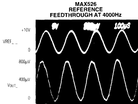
100µs/div TOP: REFERENCE IN 5V/div BOTTOM: VOUTA 200µV/div INPUT CODE - ALL 0s
