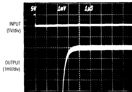
VREF = 10V, CL = 100pF, RL = 5kΩ
