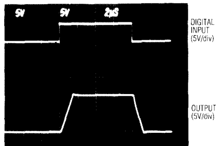
VDD = +15V, VSS = -5V, VREF = 10V, CL = 100pF, RL = 5kΩ
