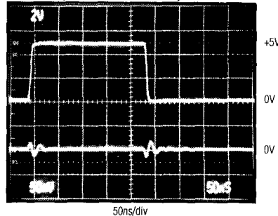
50ns/div TOP: DIGITAL TRANSITION ON ALL DATA BITS 5V/div BOTTOM: DAC OUTPUT WITH WR HIGH 50mV/div
