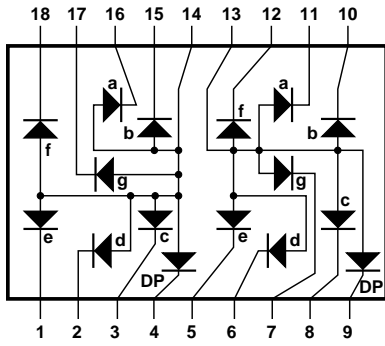
COMMON ANODE
