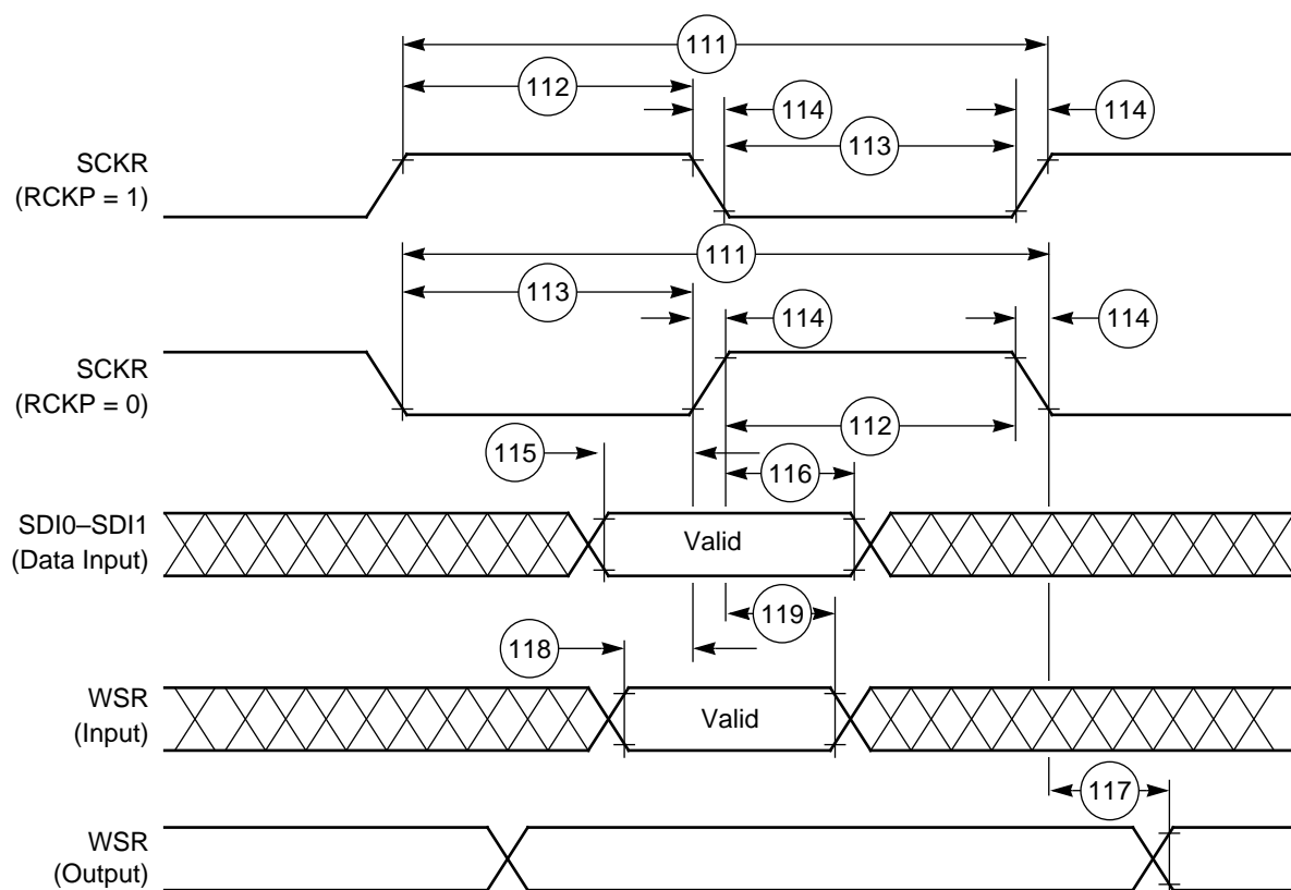
Figure 2-15 SAI Receiver Timing
