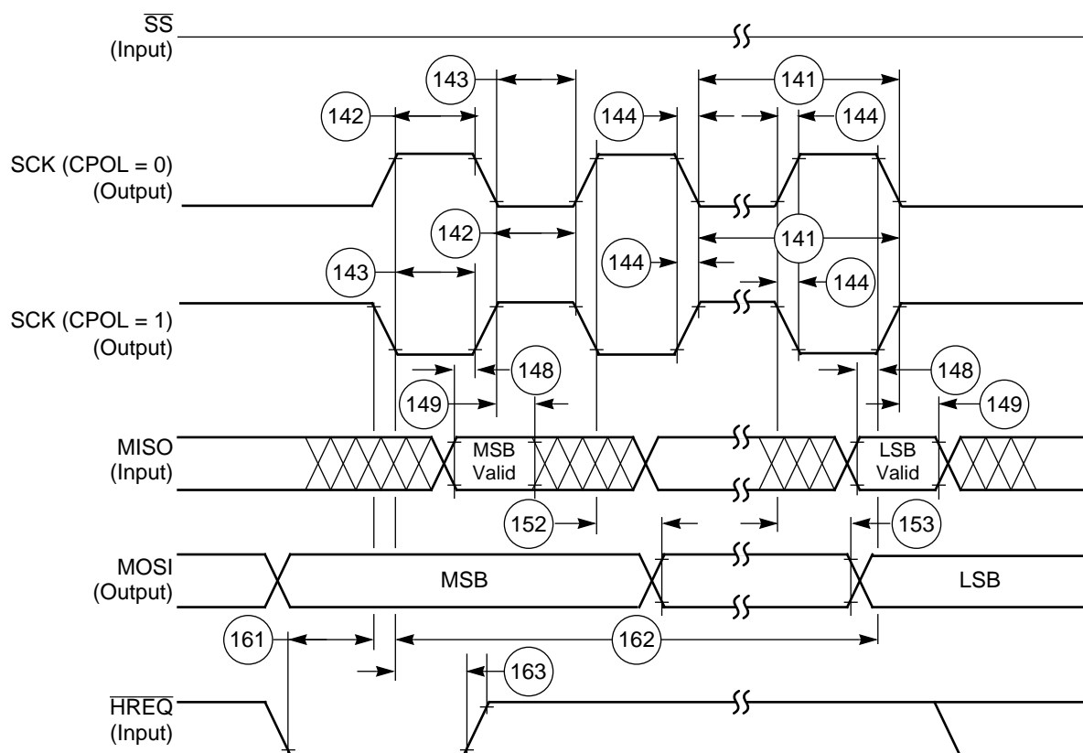
Figure 2-18 SPI Master Timing (CPHA = 1)
