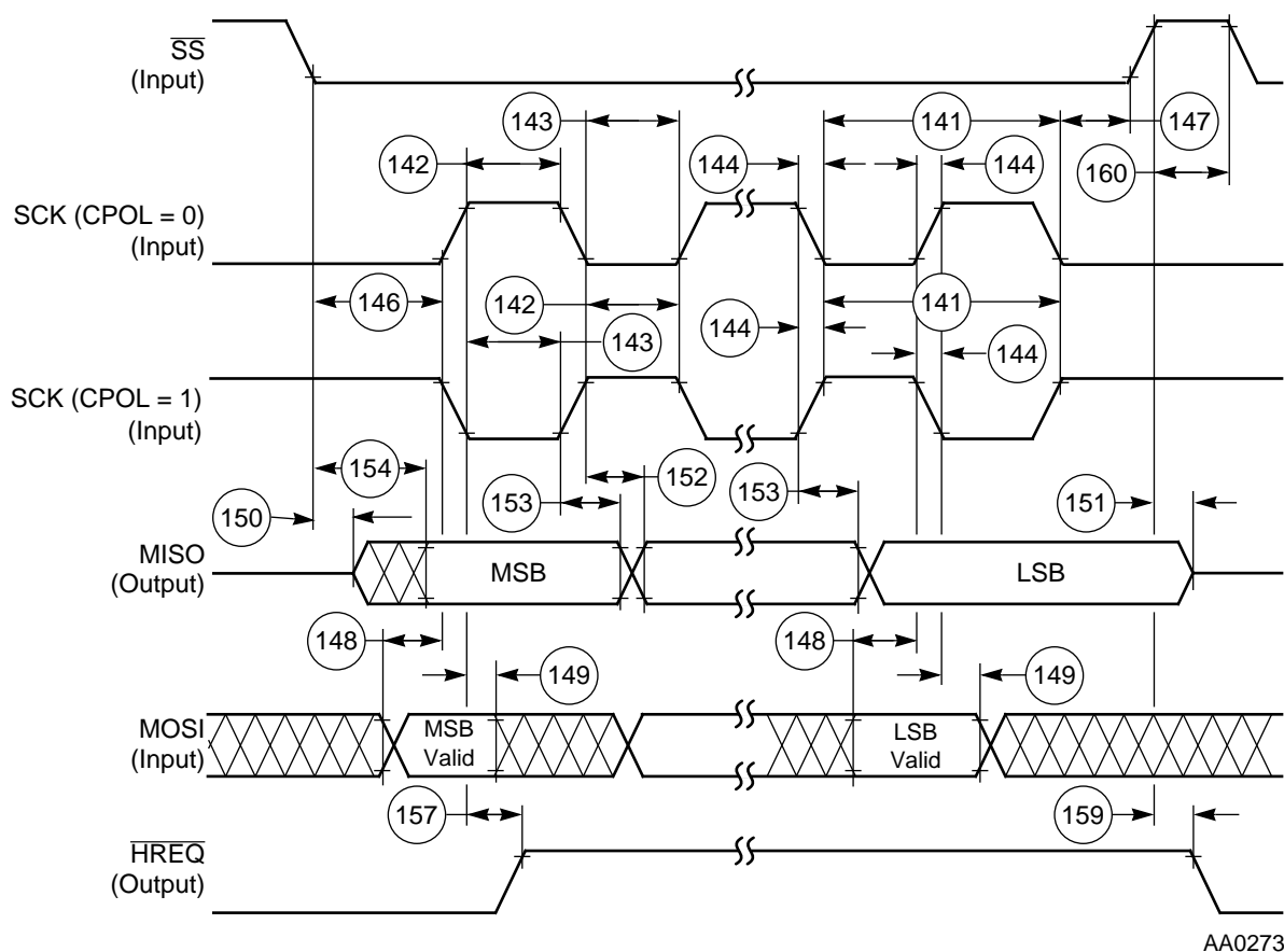
Figure 2-19 SPI Slave Timing (CPHA = 0)
