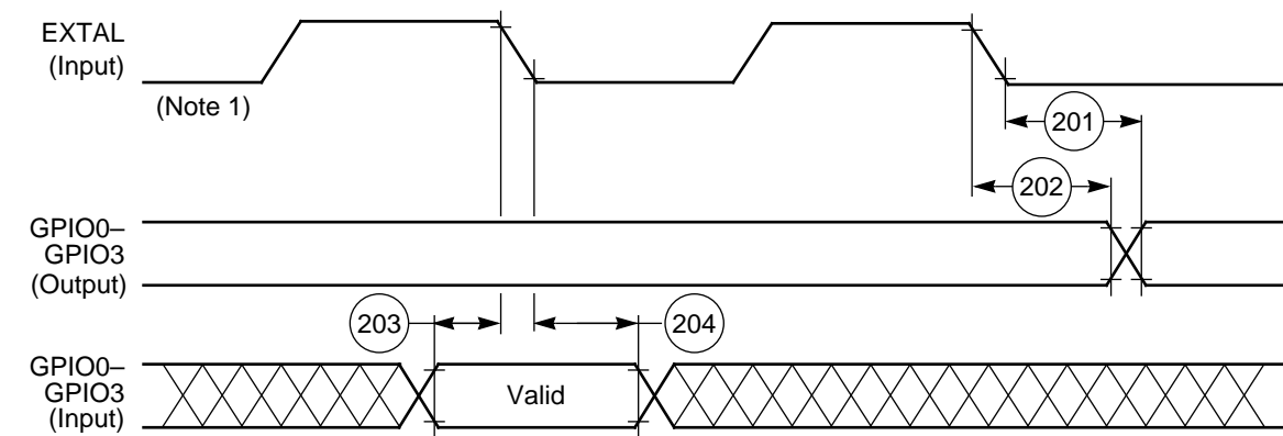
Figure 2-22 GPIO Timing
