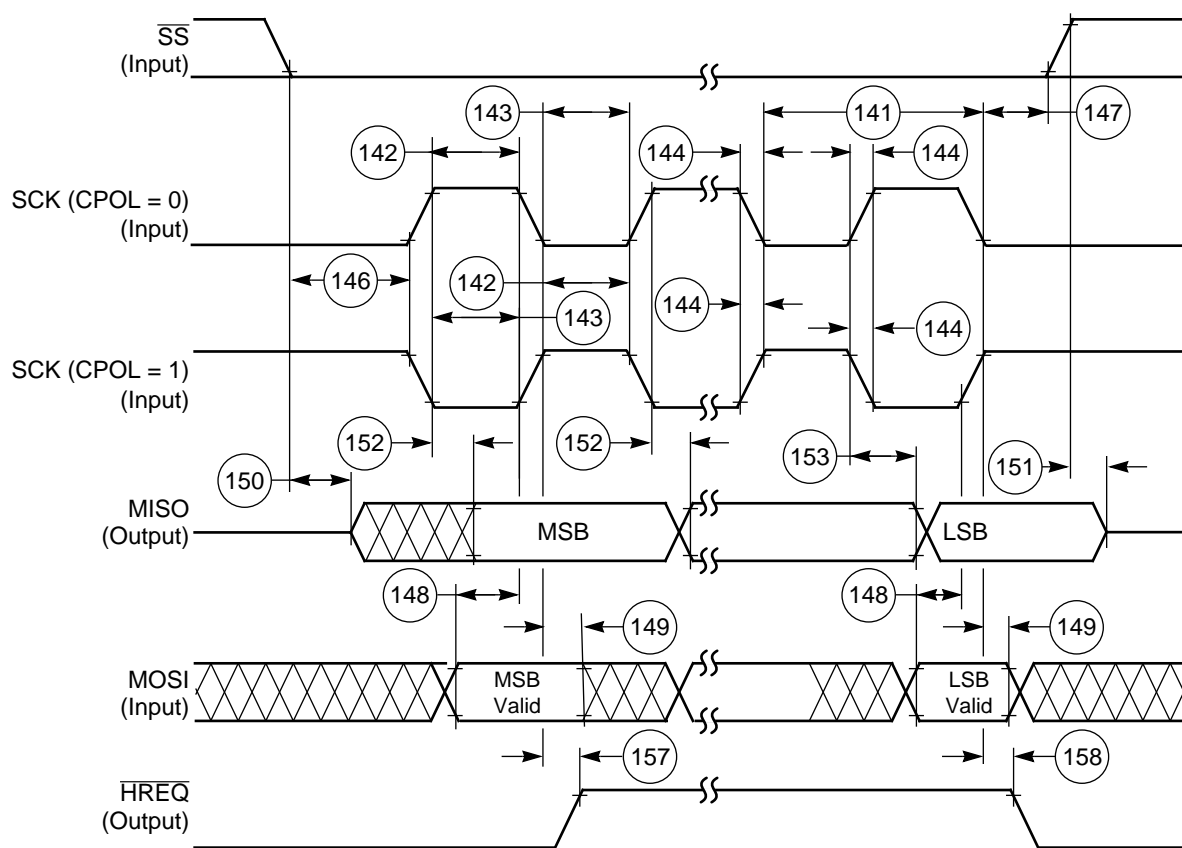
Figure 2-20 SPI Slave Timing (CPHA = 1)
