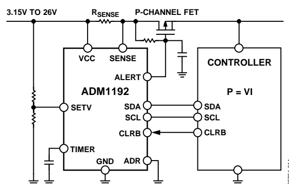
Figure 28. P-Channel FET Hot Swap Implementation
