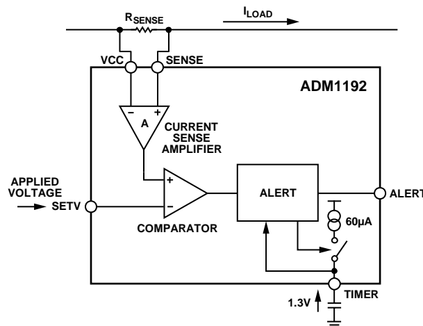
Figure 29. SETV Operation
