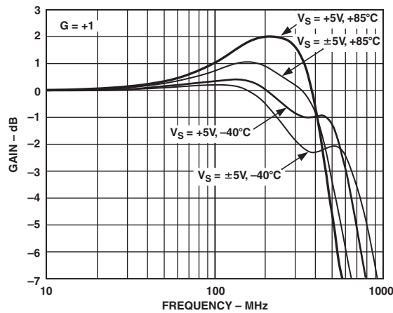
TPC 8. Small Signal Frequency Response over Temperature, V_S = +5V, \pm 5V
