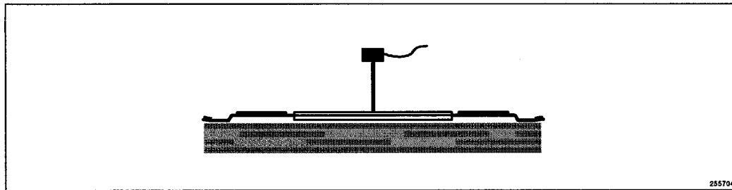
Figure 20. Technique for Measuring Case Temperature ( T_C )
