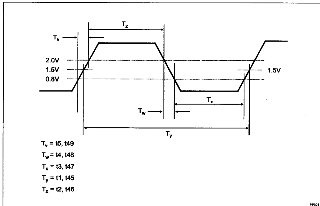
Figure 3. Clock Waveform
