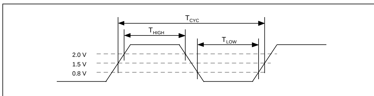
Figure 9.6 Clock Waveform
