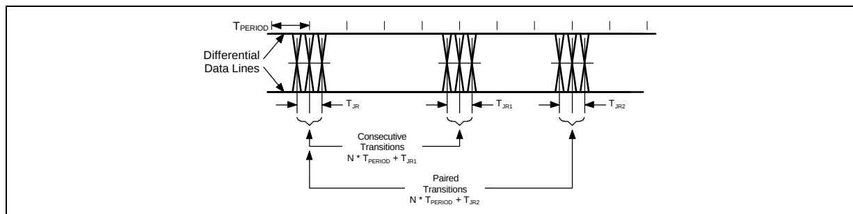
Figure 9.4 Receiver Jitter Tolerance
