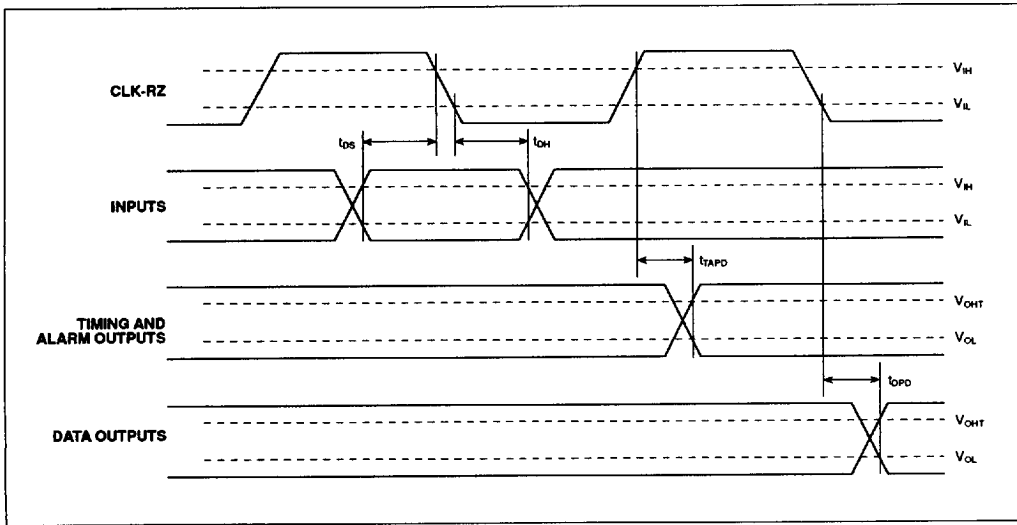
Fig. 7 Timeslot zero receiver timing
