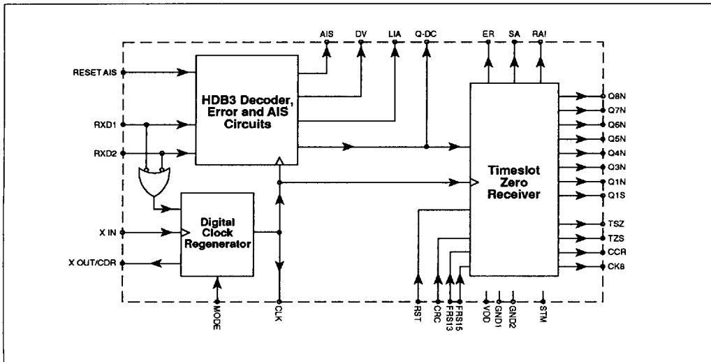
Fig. 2 Block diagram
