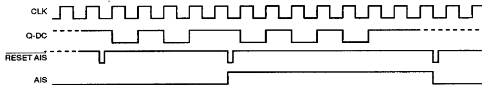
Fig. 3 HDB3 Decoder timing
