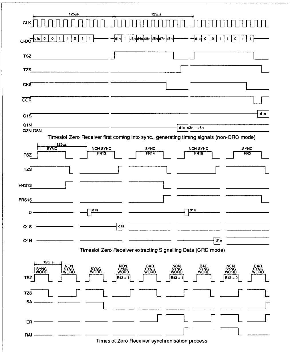
Fig. 4 Timeslot zero receiver timing
