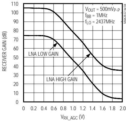
RECEIVER GAIN vs. GAIN-CONTROL VOLTAGE
