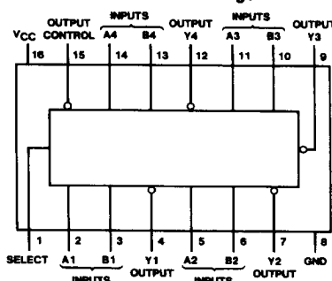
Dual-In-Line Package
