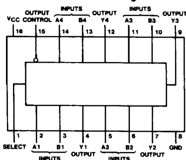
Dual-In-Line Package
