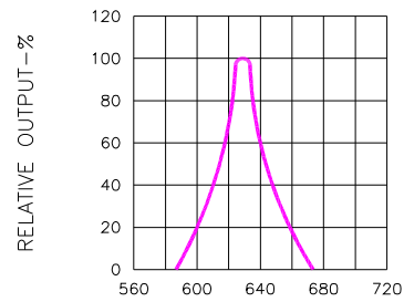
Fig.2 SPECTRAL RESPONSE
