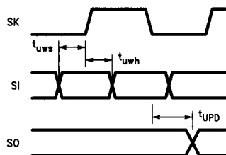
FIGURE 2. MICROWIRE/PLUS Timing
