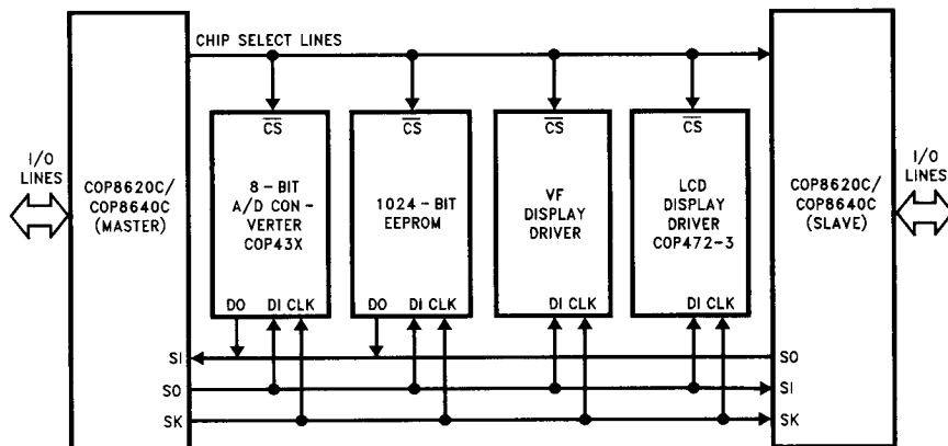
FIGURE 8. MICROWIRE/PLUS Application
