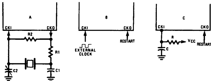
FIGURE 5. Crystal and R-C Connection Diagrams
