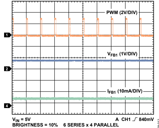
Figure 12. LED Current Waveforms (Brightness = 10%)
