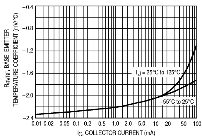
Figure 10. Temperature Coefficients
