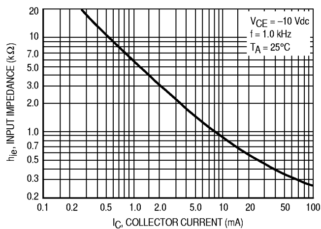
Figure 15. Input Impedance
