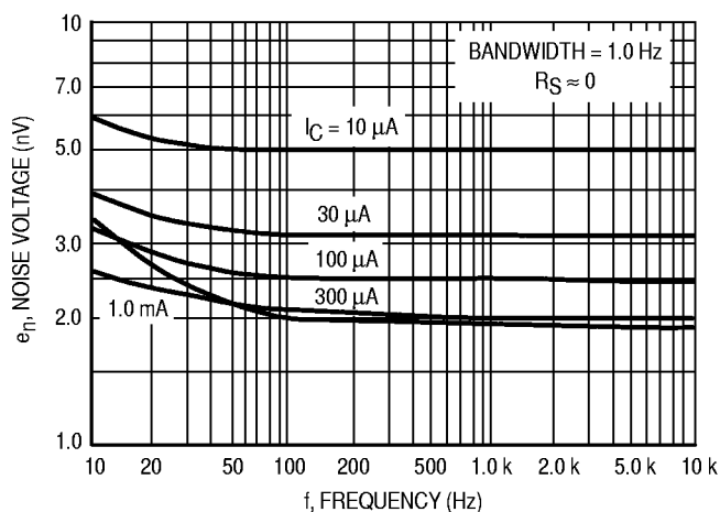
Figure 1. Noise Voltage
