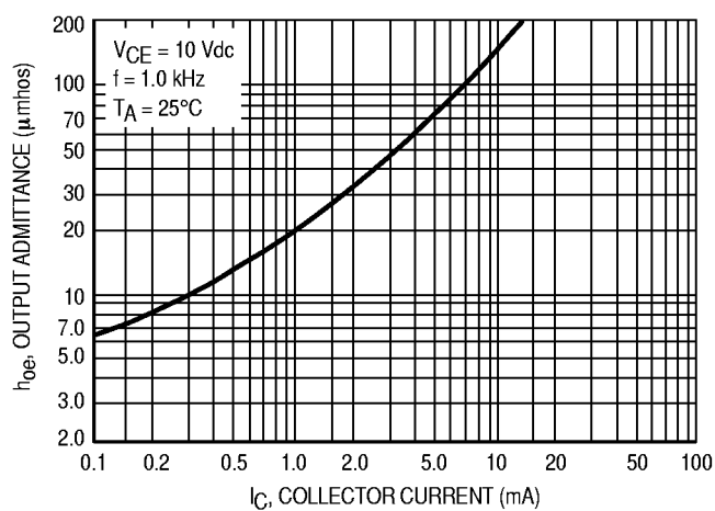
Figure 16. Output Admittance
