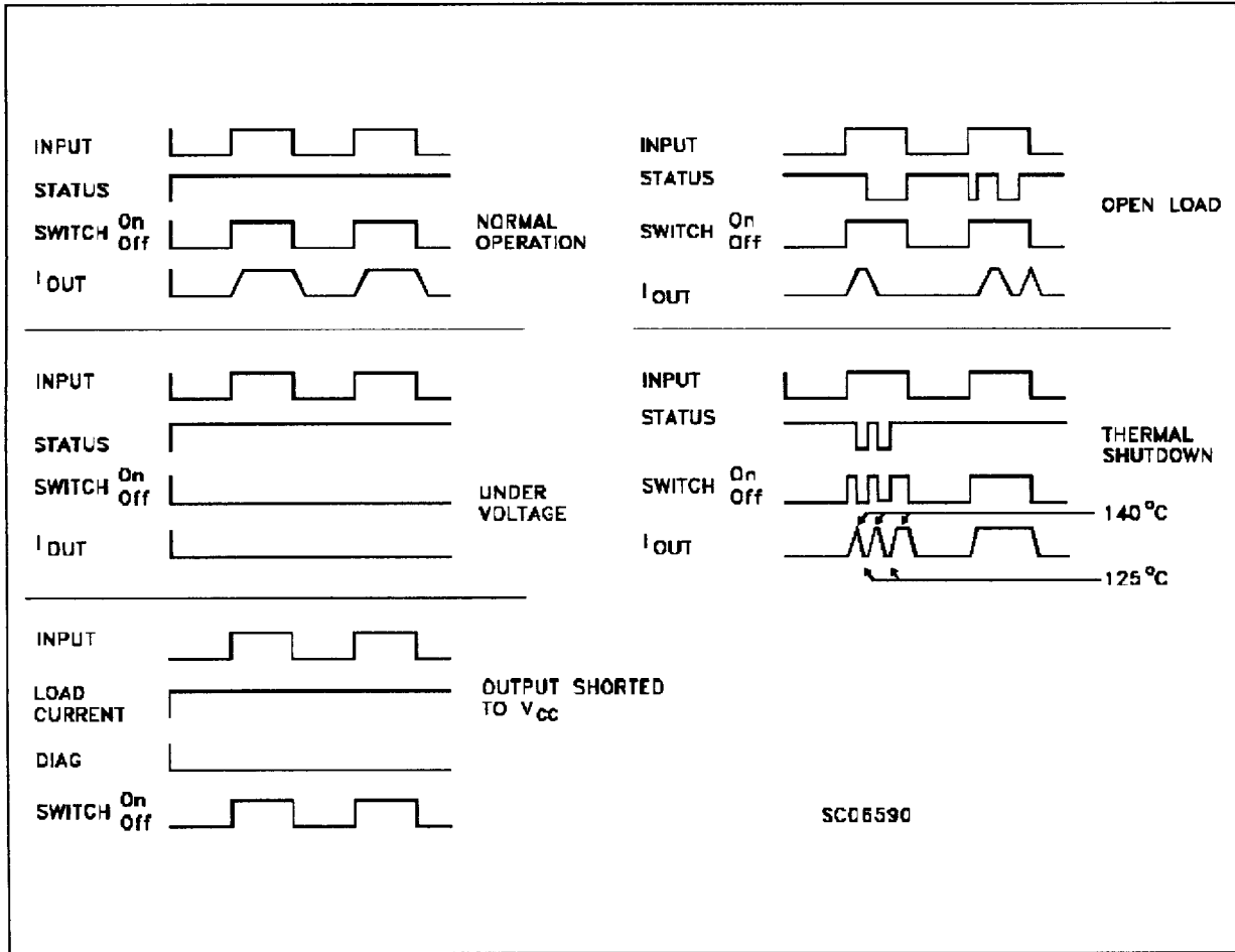
Figure 1: Waveforms
