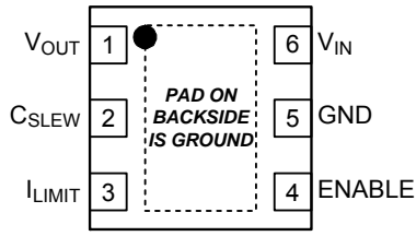
6-Pin 2mm X 2mm MLF (ML) Top View
