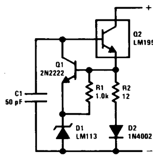
Two Terminal 100 mA Current Regulator
