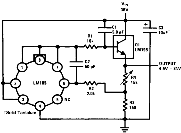
1.0 Amp Positive Voltage Regulator
