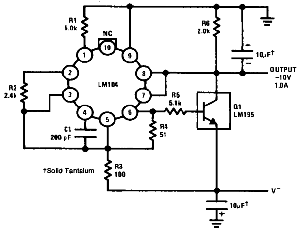
1.0 Amp Negative Regulator
