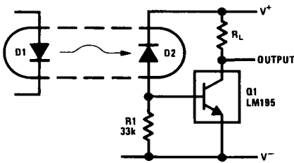
Fast Optically Isolated Switch
