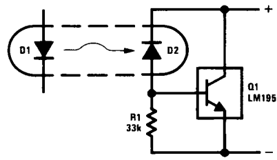
Optically Isolated Power Transistor
