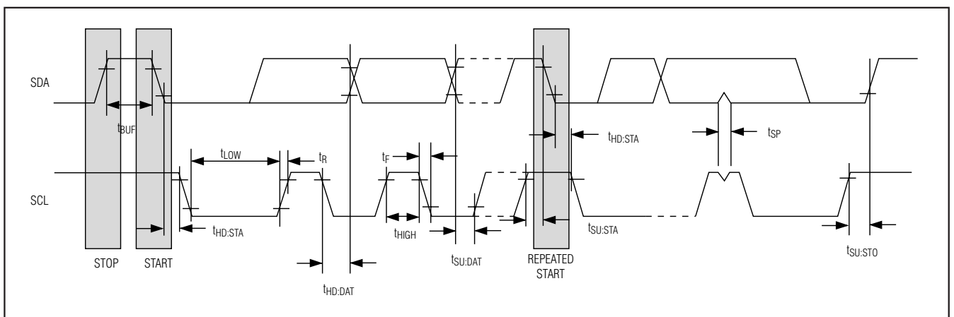
Figure 6. Timing Diagram
