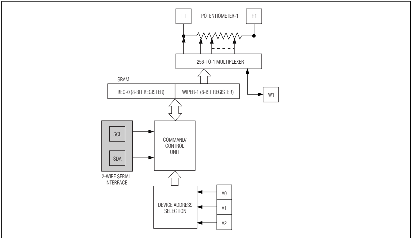
Figure 1. Functional Diagram
