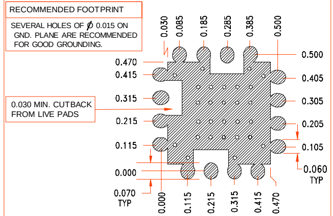
Physical Dimensions
