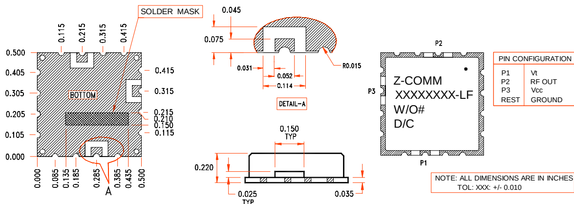
Physical Dimensions
