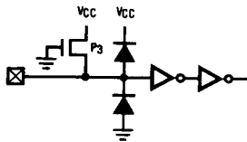
g. Input with Load
