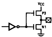
b. Low Current Push-Pull Output
