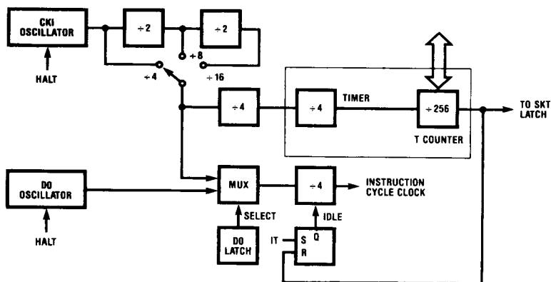
FIGURE 10B. Clock and Timer with Dual-Clock
