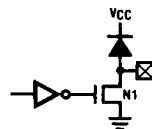
c. Open-Drain Output
