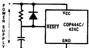
RC > 5X POWER SUPPLY RISE TIME AND RC > 100X CKI PERIOD.
