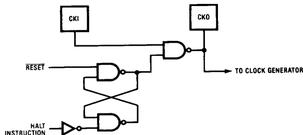
FIGURE 9A. Halt Mode — Two-Pin Oscillator
