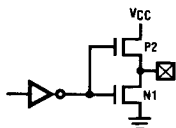
a. Standard Push-Pull Output
