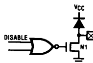
f. Open Drain TRI-STATE "L" Output
