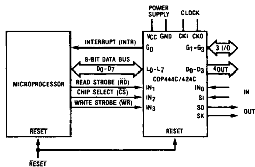
FIGURE 6. Microbus Option Interconnect
