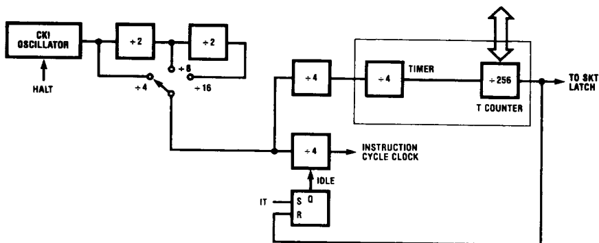
FIGURE 10A. Clock and Timer without Dual-Clock
