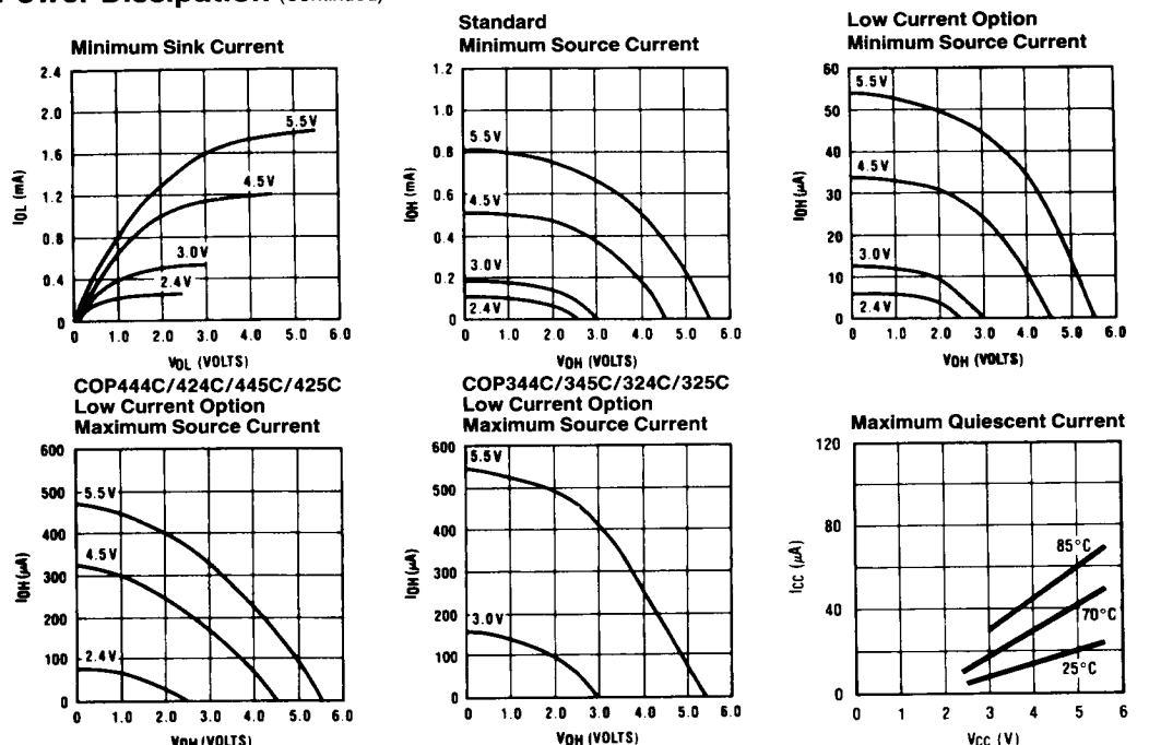
FIGURE 12. Input/Output Characteristics
