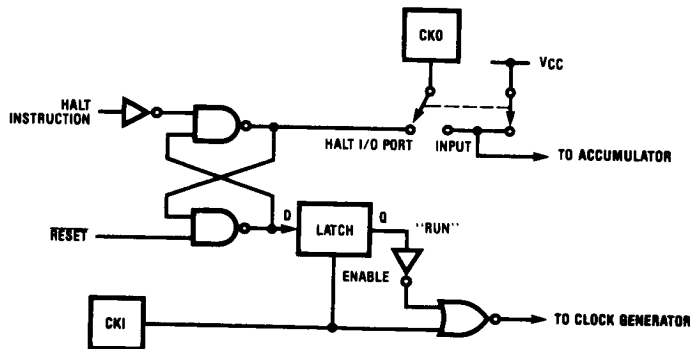
FIGURE 9B. Halt Mode — One-Pin Oscillator
