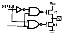
d. Standard TRI-STATE "L" Output
