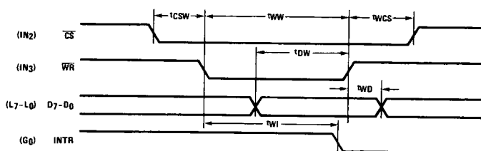
FIGURE 5. Microbus Write Operation Timing
