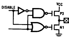
e. Low Current TRI-STATE "L" Output
