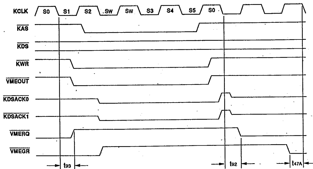
Figure 6 : DARF BUS ARBITRATION, CPU BUS REQUEST
