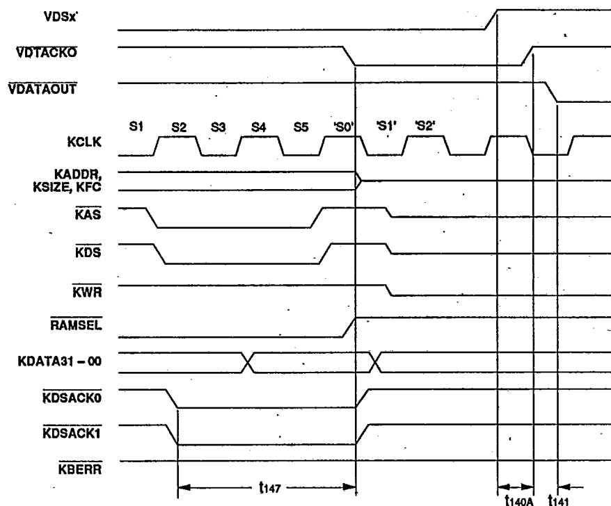
Figure 18a : DART SLAVE INTERFACE, MEMORY READ with BERRCHK CLEARED
