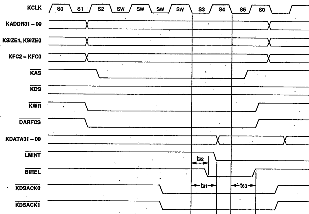
Figure 9 : DARF SLAVE INTERFACE, CPU LOCATION MONITOR WRITE
