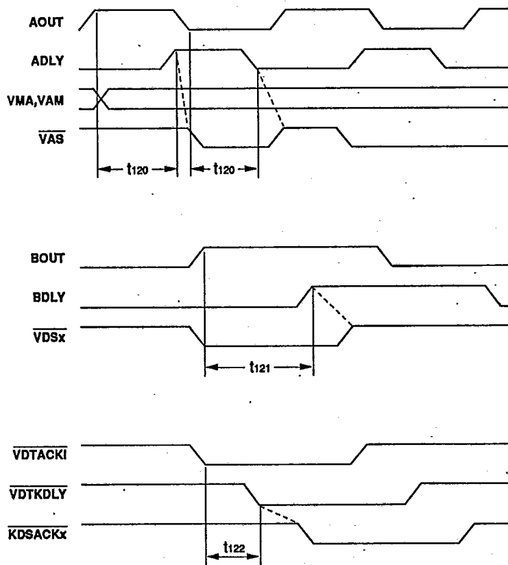
Figure 13 : DARF DELAY LINE TIMING, VMEbus MASTER CYCLES
