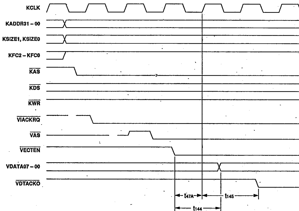
Figure 14 : DART MASTER INTERFACE, VMEbus Jack CYCLE
