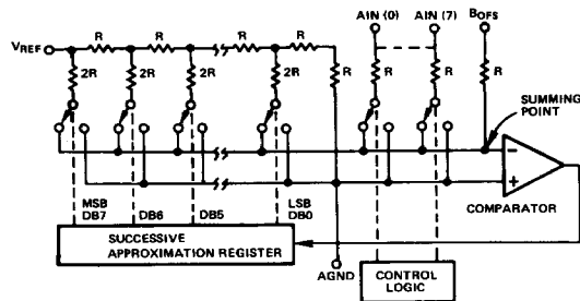
Figure 2. D/A Converter as Used in AD7581
