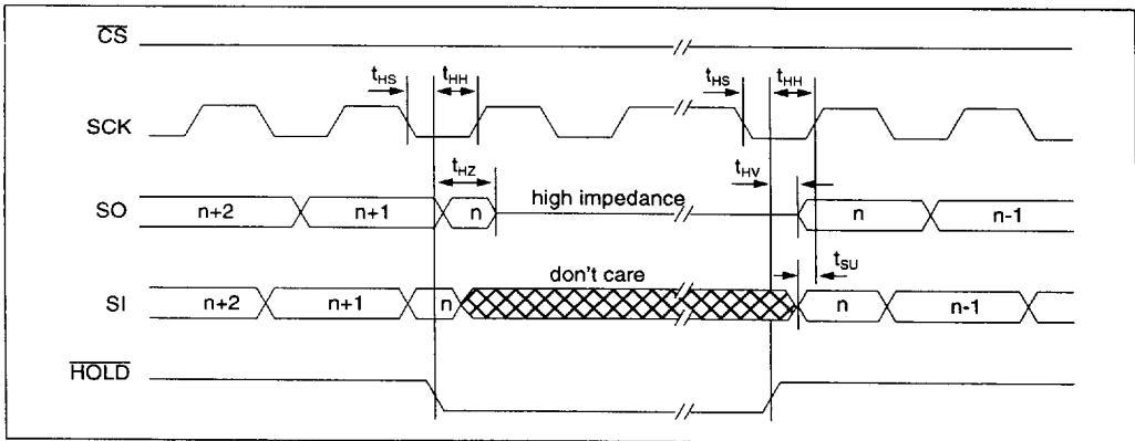
FIGURE 1-4: HOLD TIMING
