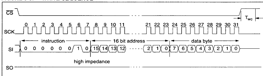
FIGURE 3-3: WRITE SEQUENCE
