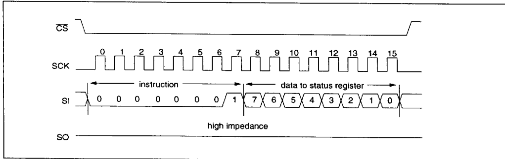
WRITE STATUS REGISTER SEQUENCE
