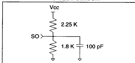
FIGURE 1-1: AC TEST CIRCUIT
