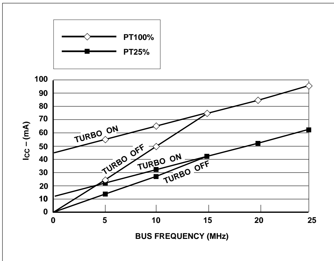
Figure 37a. ZPLD I_{CC} /Frequency Consumption
