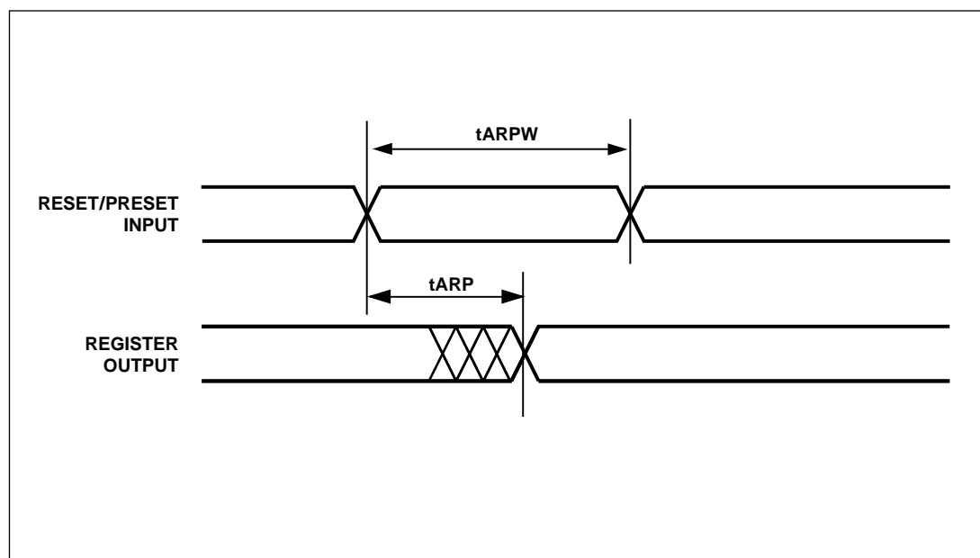
Figure 46. Asynchronous Reset/Preset
