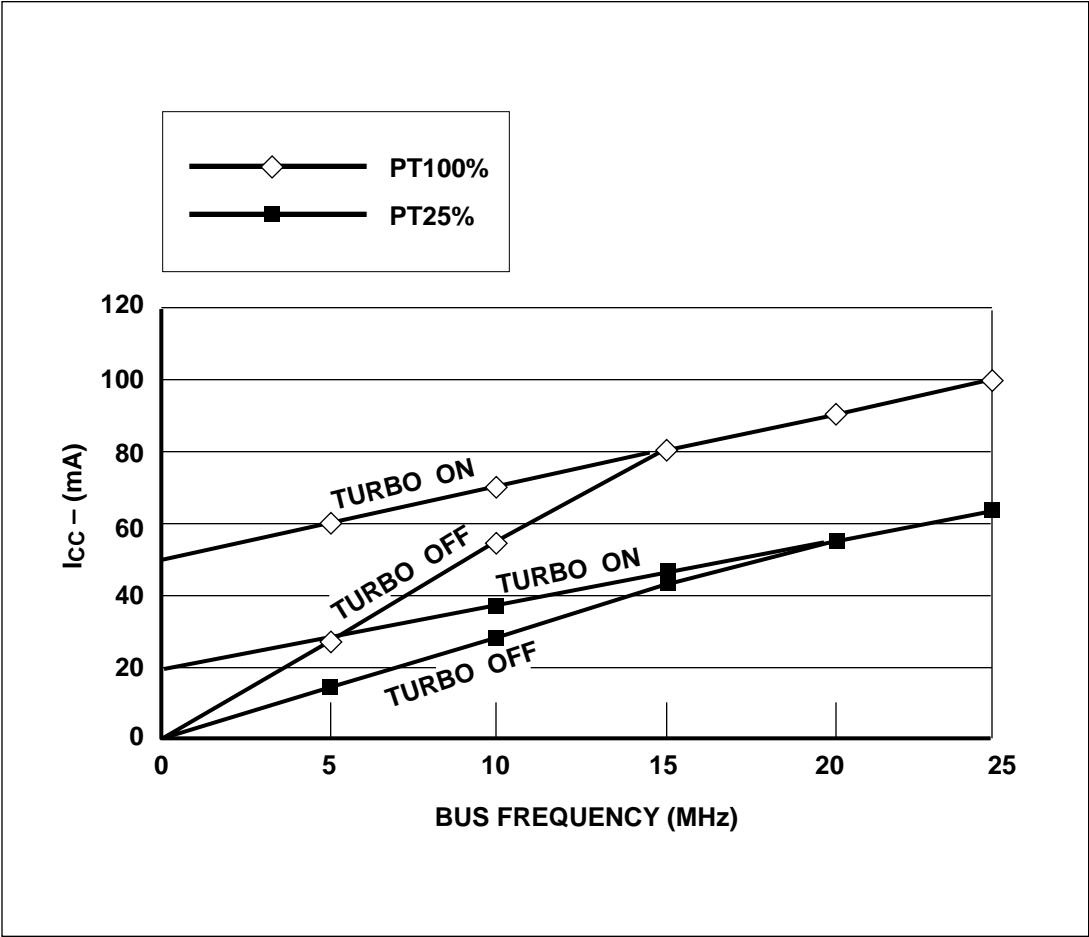
Figure 37b. ZPLD I_{CC} /Frequency Consumption
