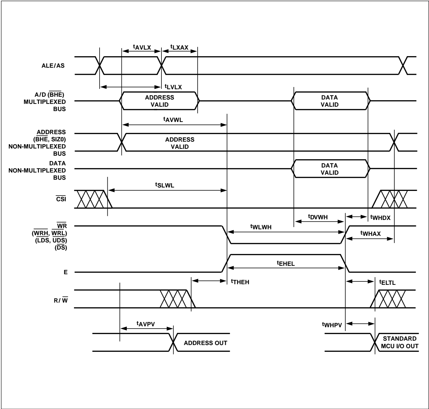
Figure 39. Write Timing
