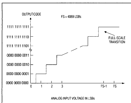
Figure 12 Ideal Unipolar Transfer Function
