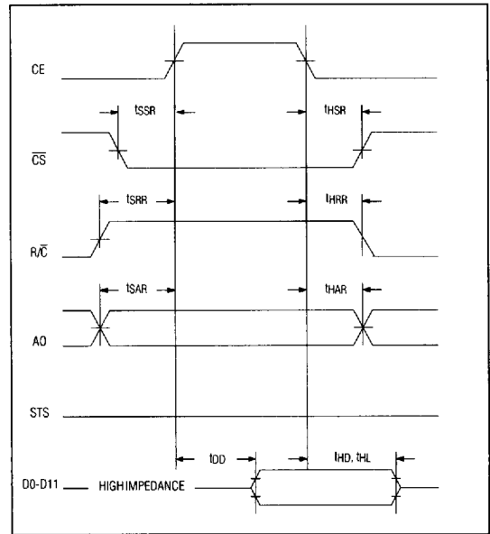
Figure 5 Read Timing
