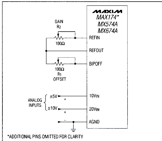
Figure 15 Bipolar Input Connections
