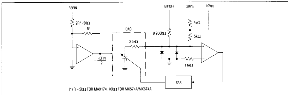
Figure 3 Analog Equivalent Circuit
