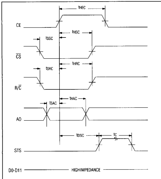
Figure 4 Convert Start Timing
