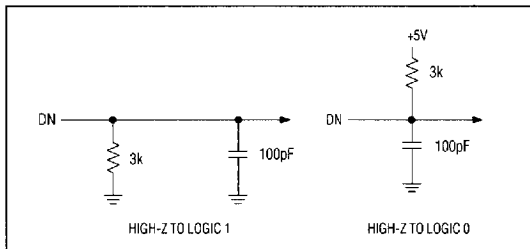
Figure 1 Load Circuit for Access Time Test
