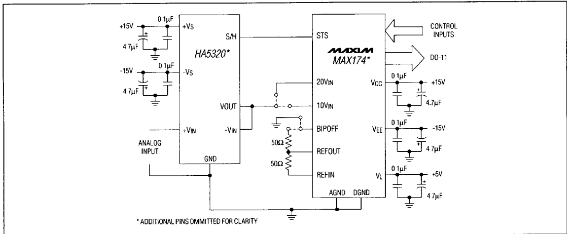
Figure 11 MAX174 to HA5320 Sample-and-Hold Interface
