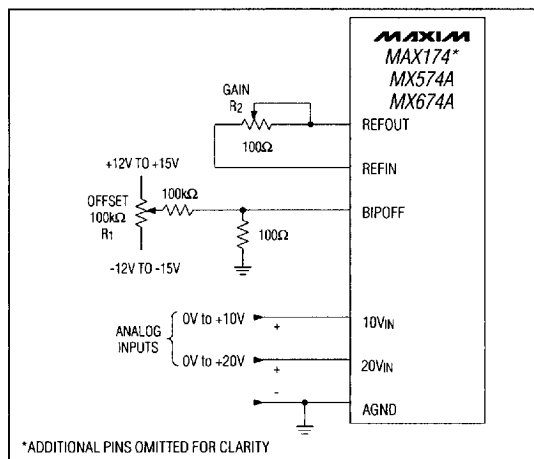
Figure 13 Unipolar Input Connections
