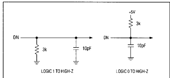
Figure 2 Load Circuit for Output Float Delay Test
