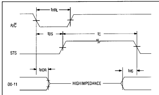
Figure 6 Low Pulse for \overline{R/C} in Stand-Alone Mode
