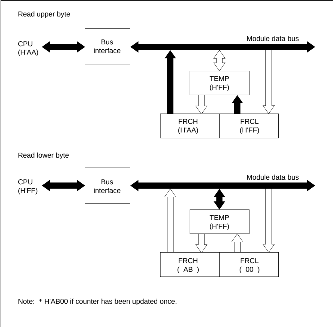
Figure 9-19 Read Access to FRC (FRC → CPU)
