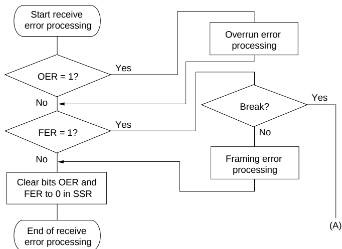
Figure 10-24 Example of Multiprocessor Data Reception Flowchart (cont)
