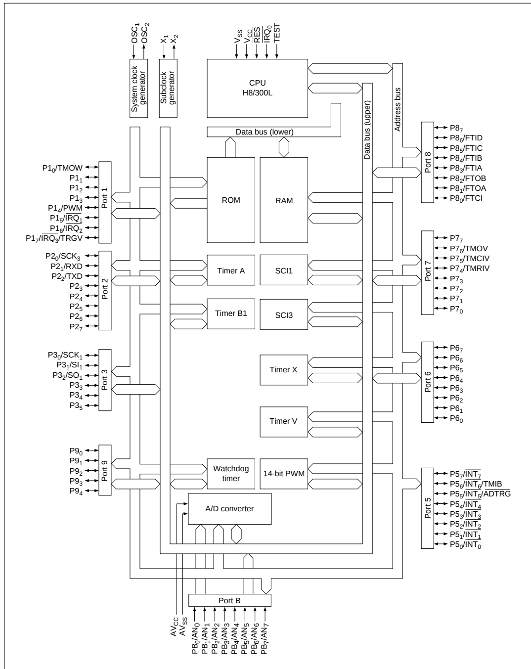
Figure 1-1 Block Diagram
