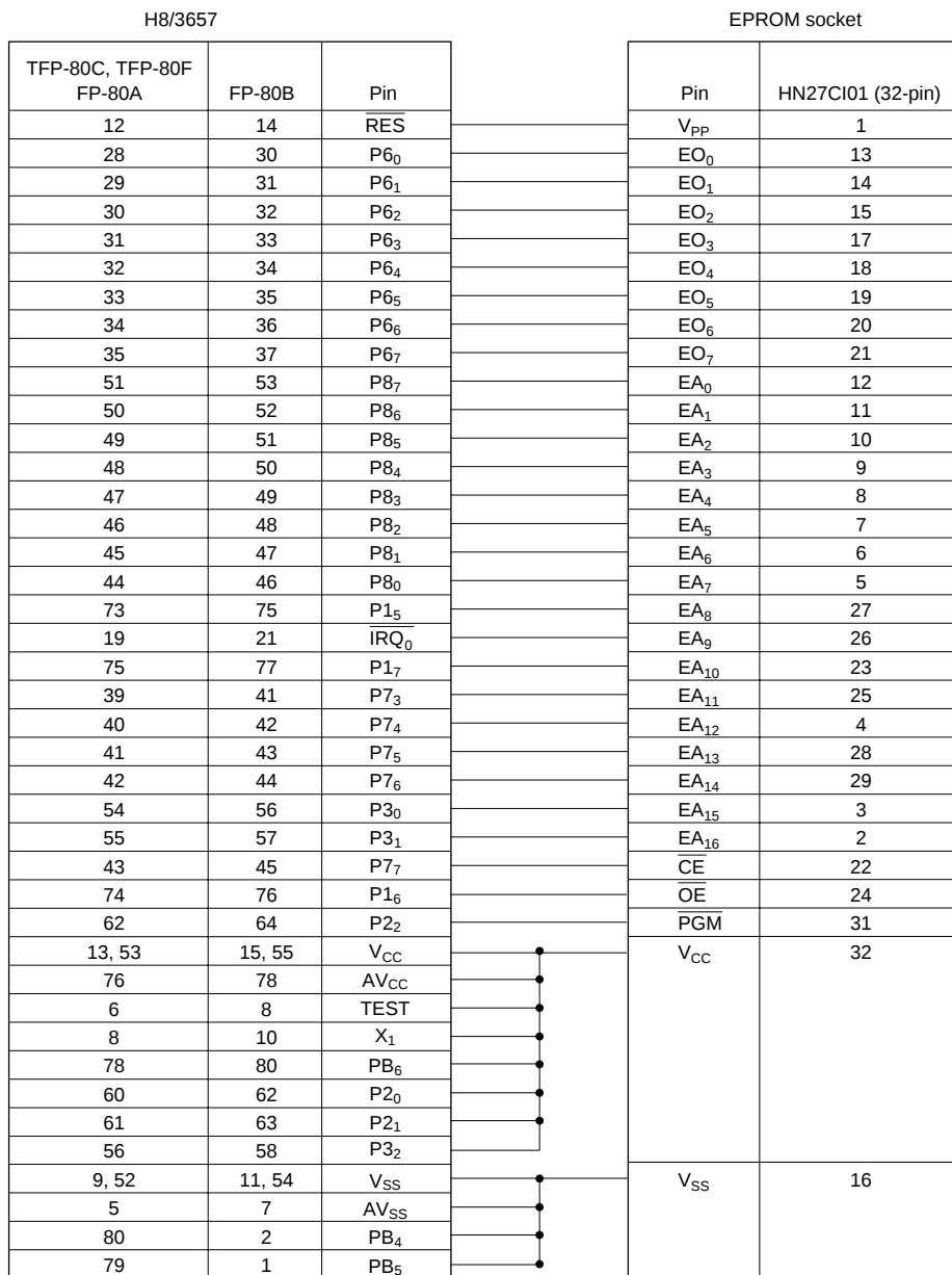
Figure 6-2 Socket Adapter Pin Correspondence (with HN27C101)
