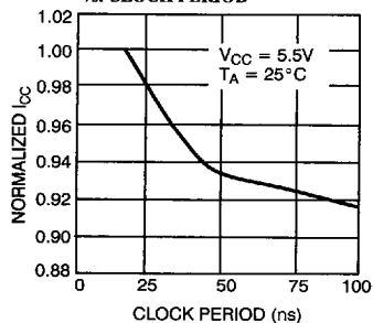
NORMALIZED SUPPLY CURRENT vs. CLOCK PERIOD
