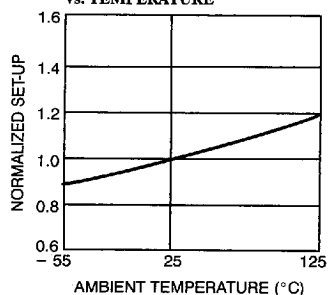
NORMALIZED SET-UP TIME vs. TEMPERATURE
