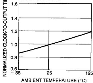
CLOCK TO OUTPUT TIME vs. TEMPERATURE
