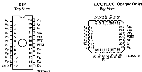
Figure 1. Programming Pinouts
