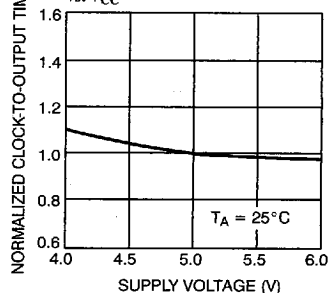
CLOCK TO OUTPUT TIME vs. V_{CC}
