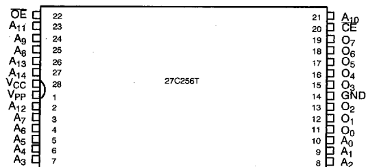
28-Pin TSOP Top View
