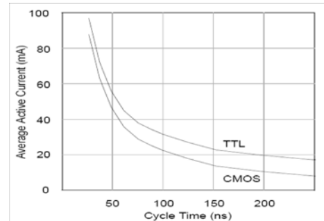
Figure 4. Current vs. Cycle Time (READ)
