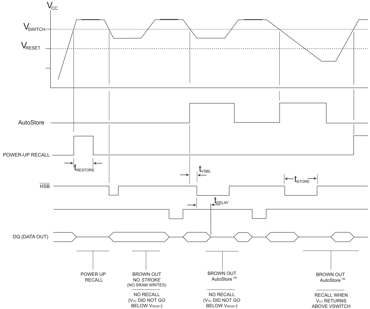
Figure 10. AutoStore/Power-Up RECALL
